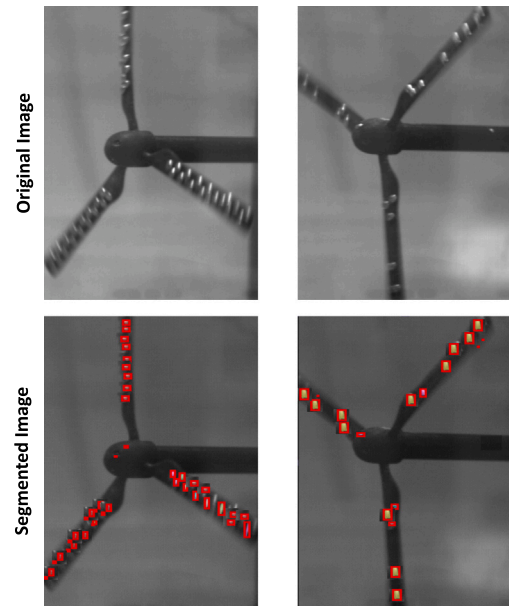
Fig. 13. Image segmentation.
