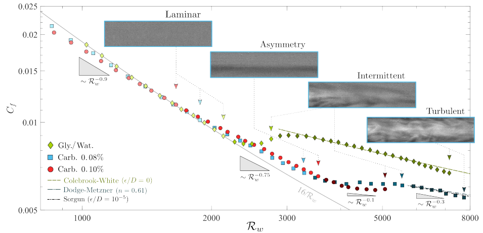
FIG. 2. Identification of flow regimes based on the friction factor C_f with the Reynolds number \mathcal{R}_w for the Carb. 0.08% (blue squares), Carb. 0.10% (red circles) and Gly./Wat. (green diamonds). For each regime (laminar, asymmetry, intermittent and turbulent), top inserts display Carb. 0.08% typical visualisation and the C_f dependence on \mathcal{R}_w is given at the bottom. Arrows indicate the end limit of the regimes. Poiseuille, Colebrook-White, Dodge-Metzner and Sorgun et al. 23 reference laws are shown to demonstrate agreements with the experimental data.
