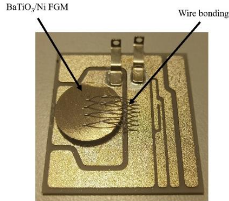
Fig. 12 \text{BaTiO}_3 FGM brazed on a substrate with wire bonding interconnections
