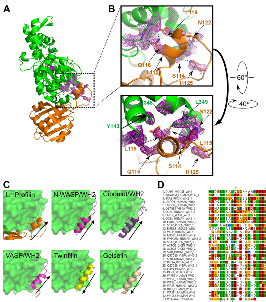
Figure 2. Trypanosomatid parasites harbor a WH2 domain-like \alpha -helical insertion. A, side view of the Leishmania profilin–actin complex showing the interactions of profilin \alpha -helical insertion with actin. B, magnified view of the interactions of Leishmania profilin \alpha -helix with actin. Key residues contributing to the interaction are marked by sticks and labeled with the same color as the corresponding protein molecule. Electron density map ( 2F_o - F_c , \sigma = 1.0 ) is also shown for selected residues. C, comparison of \alpha -helical regions of Leishmania profilin insertion (Protein Data Bank [PDB] ID: 8C47), selected WH2 domains (N-WASP/WH2 [PDB ID: 2VCP; (74)], Ciboulot/WH2 [PDB ID: 1SQQ; (75)], and VASP/WH2 [PDB ID: 2PBD; (76)]), as well as twinfilin (PDB ID: 3DAW; (77)), and gelsolin (PDB ID: 1T44; (78)). The positions of key hydrophobic residues involved in actin binding are shown. Arrows indicate the direction of polypeptide chain from the N-terminus to the C-terminus of \alpha -helix. D, multiple sequence alignment of selected WH2 domains and the \alpha -helical insertion of Leishmania profilin. The critical hydrophobic residues mediating actin monomer binding in WH2 domains are indicated with blue arrowheads. WH2, WASP homology-2 domain.
