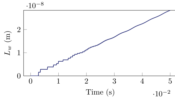
Figure 9. Wear depth
