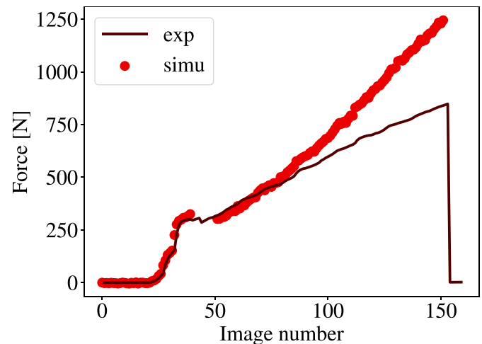
Fig. 10. Comparison between simulated (simu) and experimental (exp) reaction forces.
