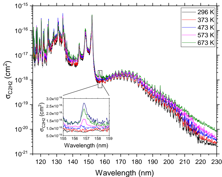
Fig. 1. Evolution of the absolute absorption cross section of C_2H_2 as a function of the temperature. Spectra were measured from 115 to 230 nm at LISA with an instrumental resolution of 0.046 nm.
