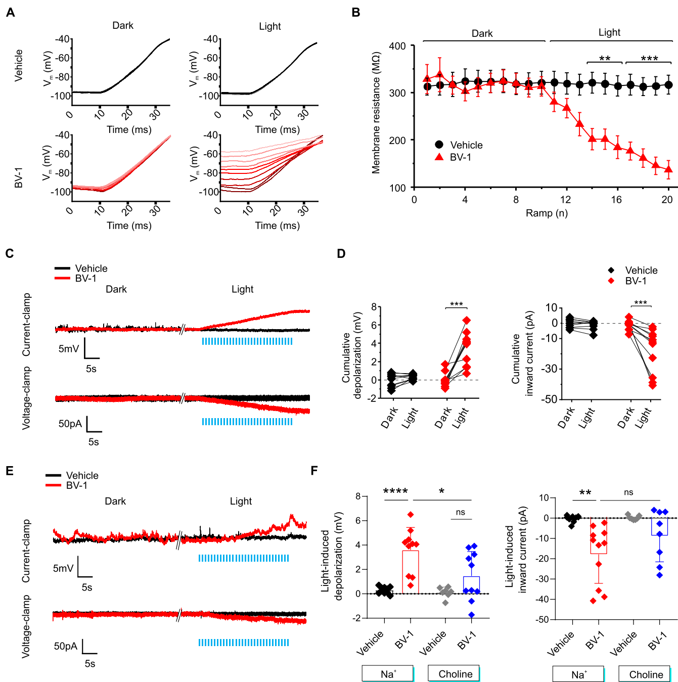
Figure 5. Light-dependent modulation of passive electrophysiological properties by BV-1. (A) Membrane voltage traces recorded with 10 CC ramps applied at 2 Hz, driving the membrane voltage from -95 to -40 mV in 20 ms in the dark and upon light stimulation (200 ms, 3 mW/mm 2 ) from neurons incubated with either vehicle or BV-1. (B) Membrane resistance calculated from the slope of the recorded voltage traces during 10 ramps in the dark and 10 ramps under light stimulation ( n = 7 and 8 for vehicle and BV-1, respectively). (C) Representative membrane voltage traces recorded in CC configuration by holding the membrane voltage of primary hippocampal neurons at -70 mV (upper traces). Corresponding current traces recorded in the voltage-clamp (VC) configuration by clamping the voltage at -70 mV (lower traces). Cells were incubated with either vehicle (H 2 O, black traces) or BV-1 (1 \mu M, red traces), and measurements were performed either in the dark or under light train stimulation (1 Hz, 20 ms, 30 light pulses, 3 mW/mm 2 ) in the presence of synaptic blockers and TTX (1 \mu M). (D) Cumulative membrane depolarization (left) and inward current intensity ( I_i ; right) modulation calculated at the end of the 40 s recorded sweeps ( n = 10 and 11 for vehicle and BV-1, respectively). (E) Na + in the external medium was replaced with choline (135 mM). Representative membrane voltage traces recorded in CC configuration by holding the membrane voltage at -70 mV (upper traces), and corresponding current traces recorded in the voltage-clamp (VC) configuration by clamping the voltage at -70 mV (lower traces). Cells were incubated with either vehicle (black traces) or BV-1 (1 \mu M; red traces), and measurements were performed either in the dark or under light pulse stimulation (1 Hz, 20 ms, 30 light pulses, 3 mW/mm 2 ) in the presence of synaptic blockers and TTX (1 \mu M) in the extracellular medium. (F) Comparison of the cumulative light-induced depolarization (left) and inward current (right) in the presence of either Na + or choline in the extracellular medium ( n = 10, 11, 7, 9 for vehicle/Na + , BV-1/Na + , vehicle/choline, and BV-1/choline, respectively). Statistics: * p < 0.05 , ** p < 0.01 , *** p < 0.001 ; two-way ANOVA/Sidak's tests (B, F); Wilcoxon's test (D).
