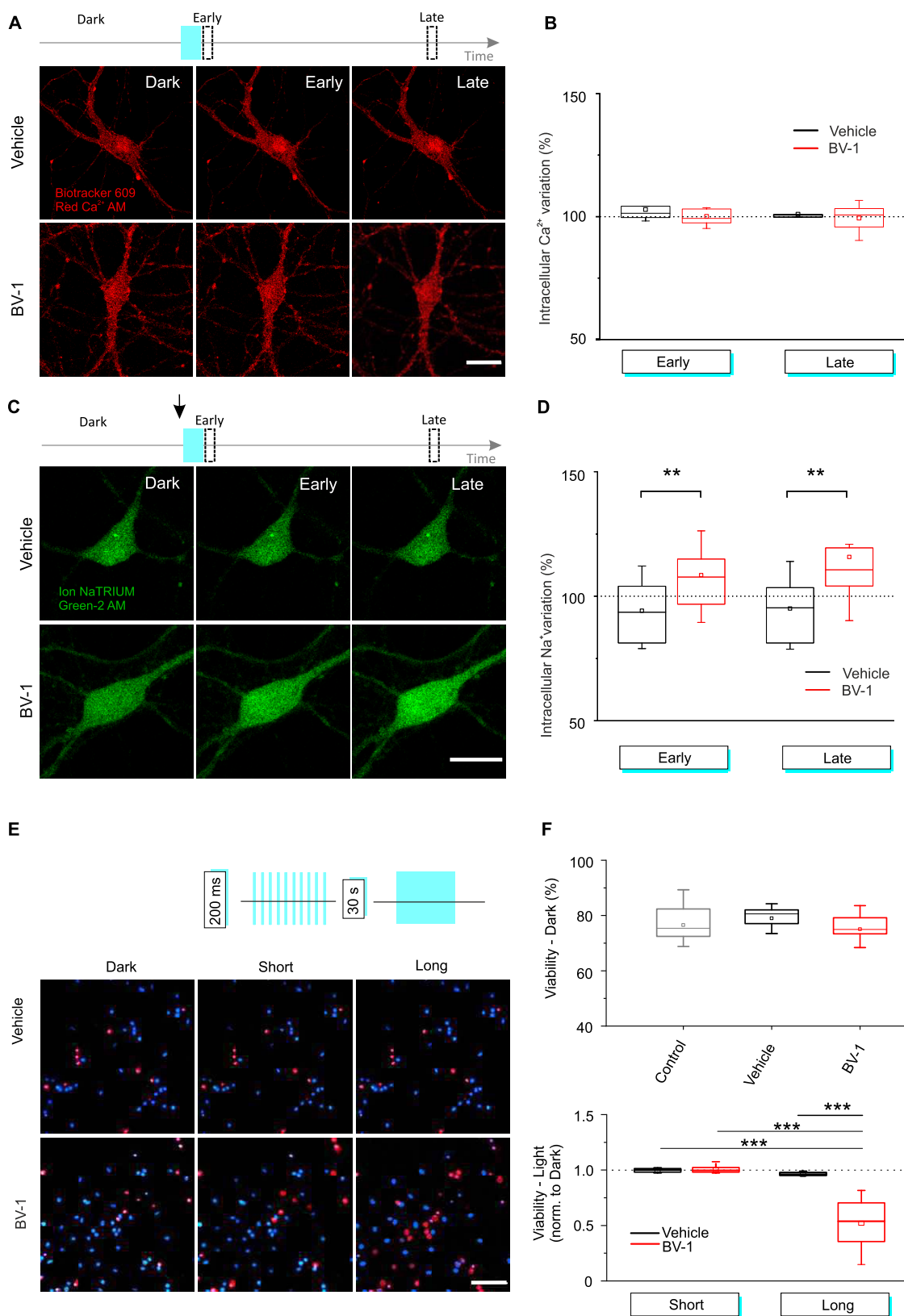
Figure 7. Light stimulation of BV-1-loaded neurons induces selective membrane permeabilization and cell death upon prolonged illumination. (A) Representative confocal images of intracellular Ca 2+ levels using a Ca 2+ fluorescent tracer (Biotracker 609 Red Ca 2+ AM) at 0 and 30 s after light stimulation. Primary hippocampal neurons were incubated with either vehicle (H 2 O, 0.1%) or BV-1 (100 nM). Ca 2+ levels were acquired immediately after (Early) and 30 s after (Late) a single-pulse light stimulation (3 s at 3 mW/mm 2 ). All acquisitions were performed in the presence of synaptic blockers and TTX (1 μM) in the extracellular medium. Scale bar, 20 μm. (B) Quantification of the early and late changes in intracellular Ca 2+ levels. The fluorescence increases of the Ca 2+ tracer upon light stimulation were normalized by the fluorescence levels in the dark ( F/F_0 \times 100 ) ( n = 5 and 11 for vehicle and BV-1, respectively). (C) Representative confocal images of
