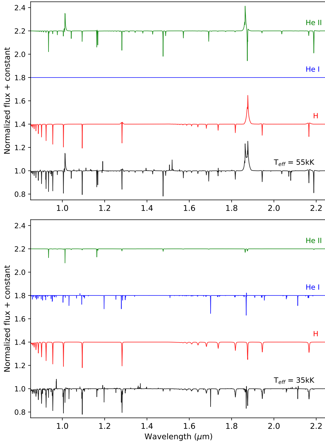
Fig. A.3. Examples of infrared spectra at 0.85–2.25 μm (LMC metallicity). Top panel: model with T_{\text{eff}} = 55 kK and \log g = 4.0 . Bottom panel: model with T_{\text{eff}} = 35 kK and \log g = 4.0 . The spectra were convolved with R = 2700 , appropriate, for example, for JWST NIRSpec data. In each panel, the full spectrum is shown at the bottom (black) and individual H I, He I, and He II contributions are denoted above.
