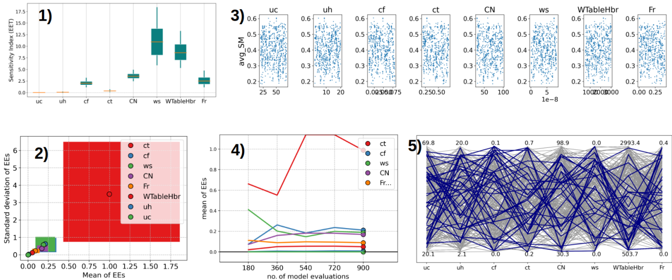
Figure A1. Diagnostic plots of the GSA: (1) sensitivity index of the perturbed parameters, (2) mean versus standard deviation of each parameter, (3) scatterplot of the sampled parameters, (4) convergence, and (5) behavioral runs (here based on the threshold KGE > 0.5 ).
