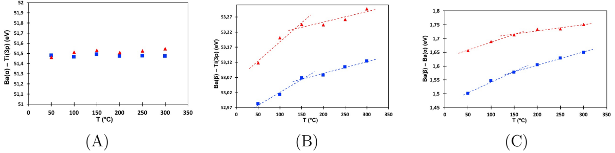
Figure 5: Experimental evolution of binding energy differences of (A) |Ba(\alpha) - Ti\ 3p| (B) |Ba(\beta) - Ti\ 3p| and (C) |Ba(\alpha) - Ba(\beta)| as a function of temperature (in °C). Values for sample 1 (10 nm of BaTiO 3 ) are reported with blue squares, while red triangles stand for sample 2 (16 nm of BaTiO 3 ). Dotted lines are linear regression used as eye guidelines below or above 150°C.
