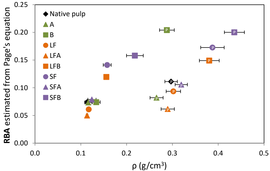
Fig. 6 Relative Bonded Area RBA estimated from Eq. (1) as a function of paper density \rho for all the monolayered model papers. Marks with a letter “P” indicate papers that were pressed upon processing.
