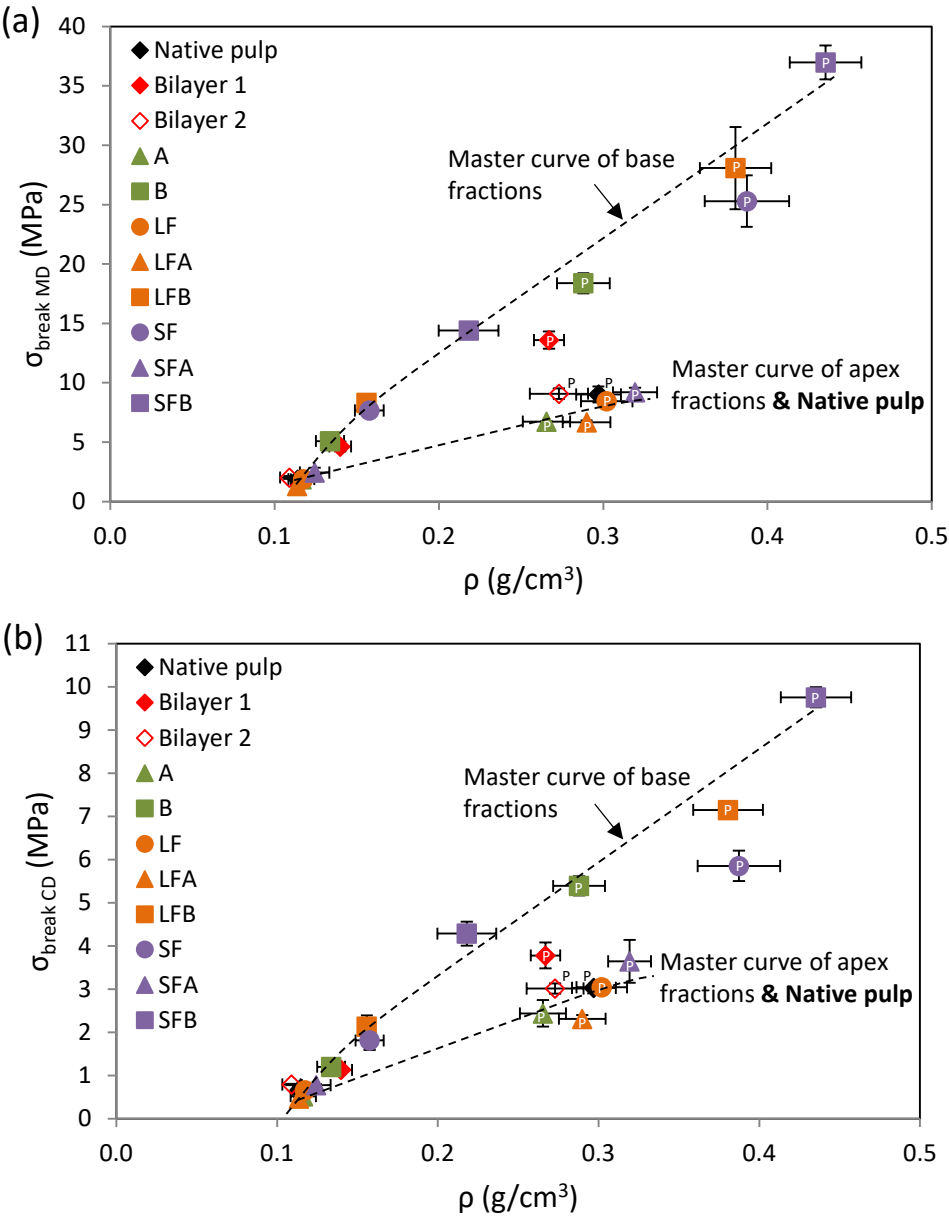
Fig. 8 Evolution of the tensile breaking stress \sigma_{break} with the paper density \rho for all model papers along the machine (a) and cross (b) directions. Marks with a letter “P” indicate papers that were pressed upon processing.
