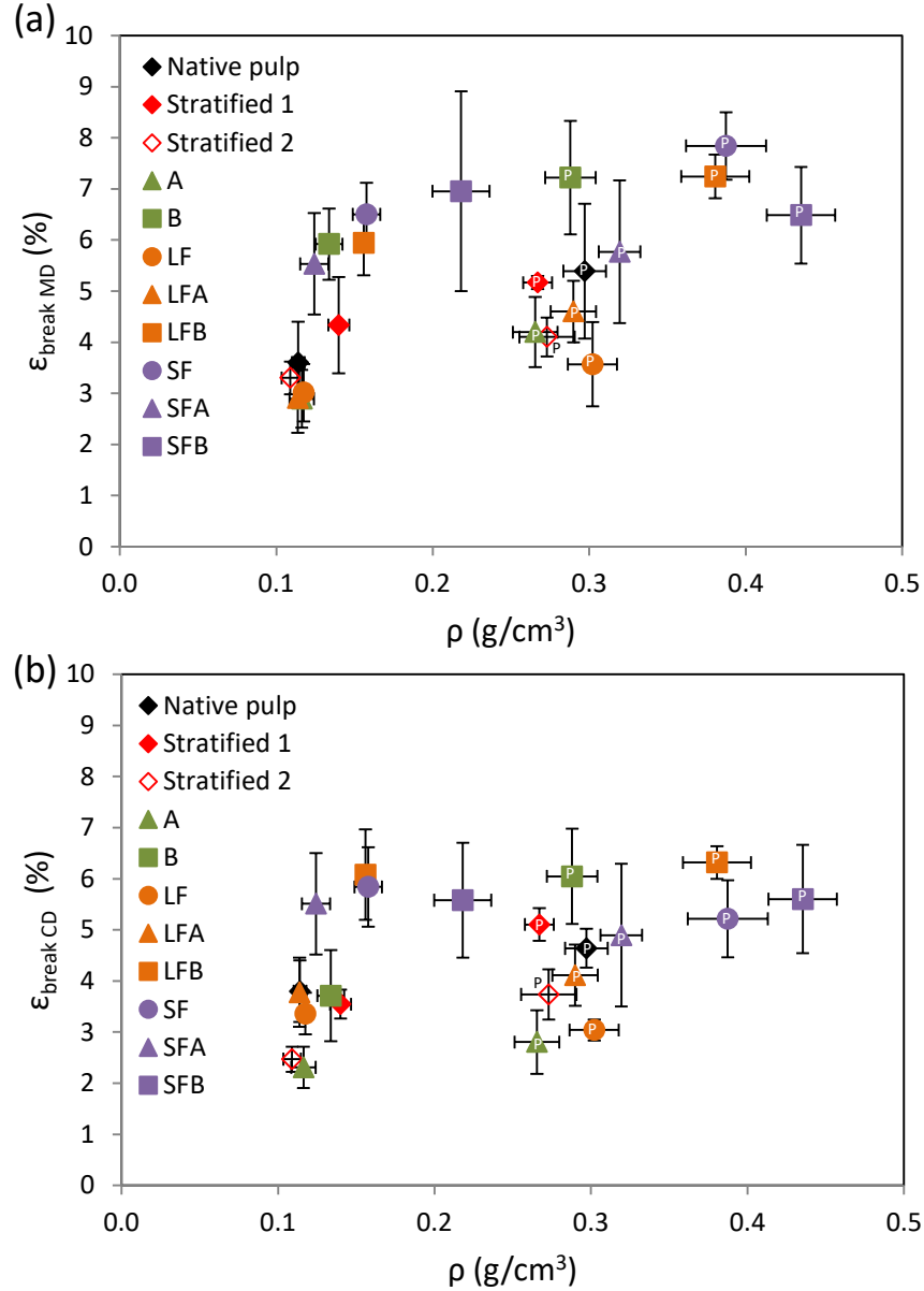
Fig. 7 Strain at break \epsilon_{break} as a function of the paper density \rho for all model papers in the (a) machine direction MD and (b) cross direction CD. Marks with a letter “P” indicate papers that were pressed upon processing.
