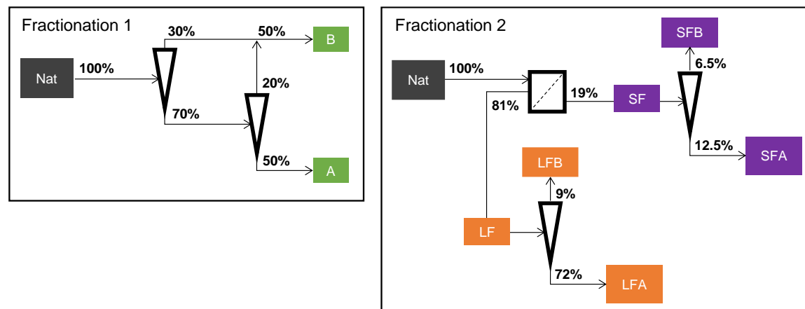
Fig. 1 – Schemes of the studied fractionation processes. Nat = Native pulp, A = Apex fraction, B = Base fraction, LF = Long Fiber fraction, SF = Short Fiber fraction, LFA = Long Fiber Apex fraction, LFB = Long Fiber Base fraction, SFA = Short Fiber Apex fraction and SFB = Short Fiber Base fraction. The percentage corresponds to the proportion of dry mass for each obtained fraction.
