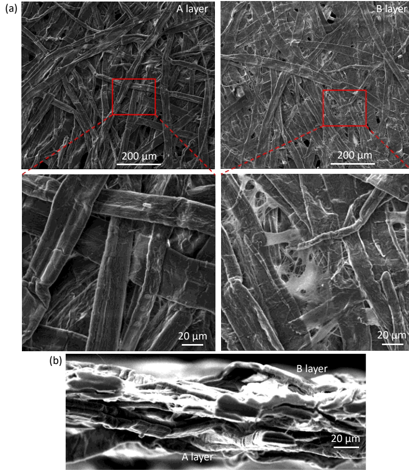
Fig. 4 FESEM micrographs of Stratified 1(A/B) paper: (a) A and B surfaces, and (b) cross section.
