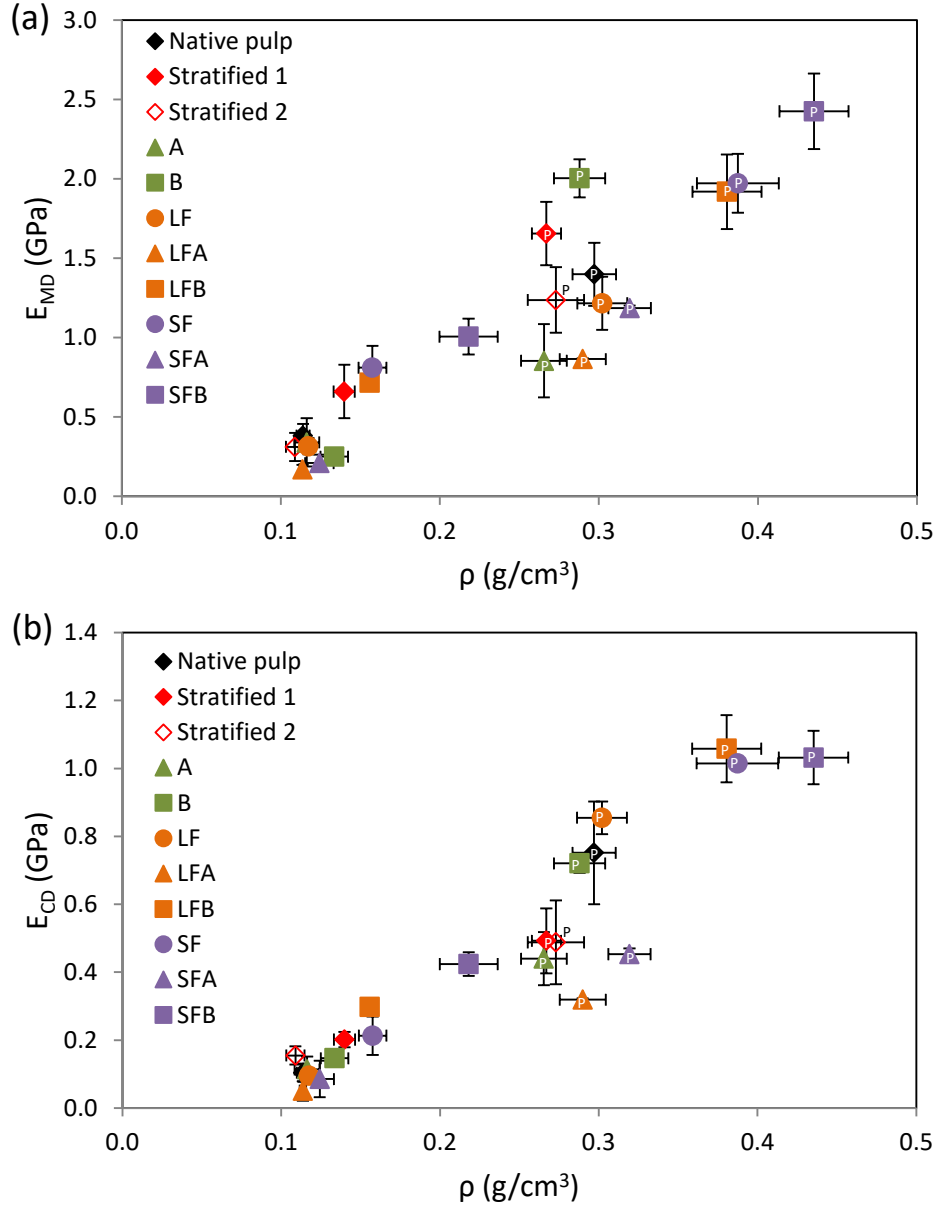
Fig. 5 Apparent Young's moduli E_{MD} (a) and E_{CD} (b) as functions of the paper density \rho for all model papers along the machine (a) and cross (b) directions. Marks with a letter "P" indicate papers that were pressed upon processing.
