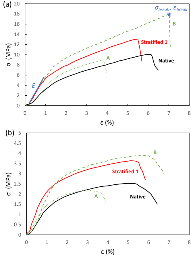
Fig 2. Representative stress-strain curves for selected model papers under pressed conditions, tested in (a) MD and (b) CD. E refers to the apparent Young’s modulus, \sigma_{break} denotes the tensile breaking stress, and \epsilon_{break} represents the strain at break.
