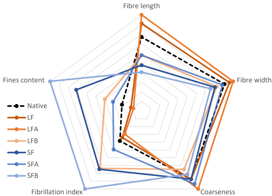
Fig 3. Comparison of the dimensionless morphological property for native pulp elements and the different fractionized pulps obtained from Approach 2. Each dimensionless property value was calculated as the ratio of the value for the respective fraction to the highest measured value.
