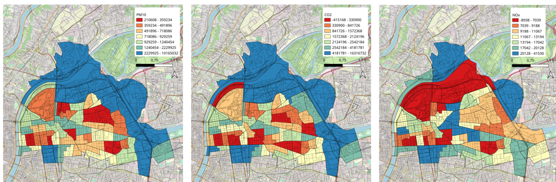
Figure 4: Spatial distribution of the gap of PM10 (left), CO2 (middle) and NOx (right) between the emissions computed from Symuvia and MATSim.
