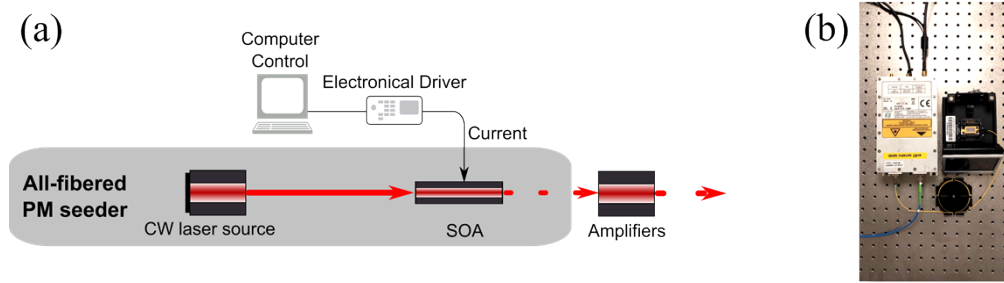
Fig. 1. (a) Schematics of an SOA used as an all-fibered temporal-shaper MOPA seeder. (b) Picture of the compact, integrated all-fibered optical arbitrary waveform generator SOA system used in this experiment. On the right, a distributed feedback narrow-linewidth (DFB) laser diode with 100 kHz linewidth and an SMSR of 45 dB, on the left, an SOA modulator. The optical signal in the seeder system is transmitted by PM980-fibers to be simply injected at the input of the chain (free space injection not shown in the picture)
