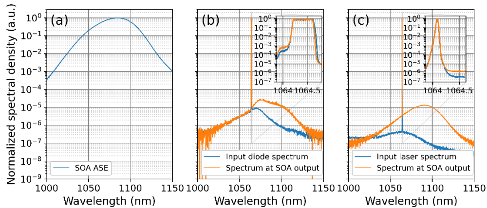
Fig. 2. Normalized spectrum measurements of (a) ASE of the SOA alimeted with current of 300 mA. The shift in central wavelength versus current is negligeeable (<1 nm over the full current dynamic) compared to the bandwidth of the ASE (b) Pulsed laser diode with a spectrum width of 0.42 nm FWHM at the SOA input and at the SOA output after temporal modulation (c) of the DFB laser at the SOA input and at the SOA output after temporal modulation. Both spectrum widths are below the OSA resolution of 0.03 nm
