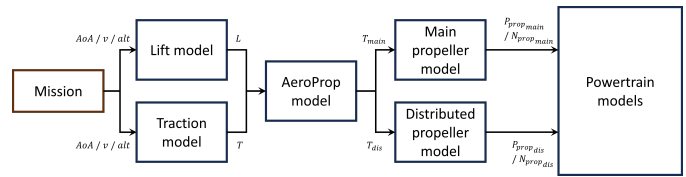
Fig. 3. Aircraft modelling workflow
