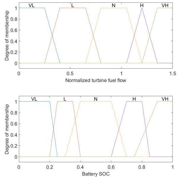
Fig. 6. SCS fuzzy logic input
