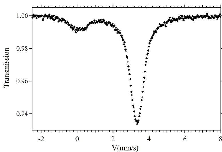
Figure 8. ^{119}\text{Sn} Experimental spectrum of \text{SnBi}_2\text{Te}_4 at 15 K. The broadened component close to 0 \text{ mm s}^{-1} is attributed to \text{SnO}_2 .
