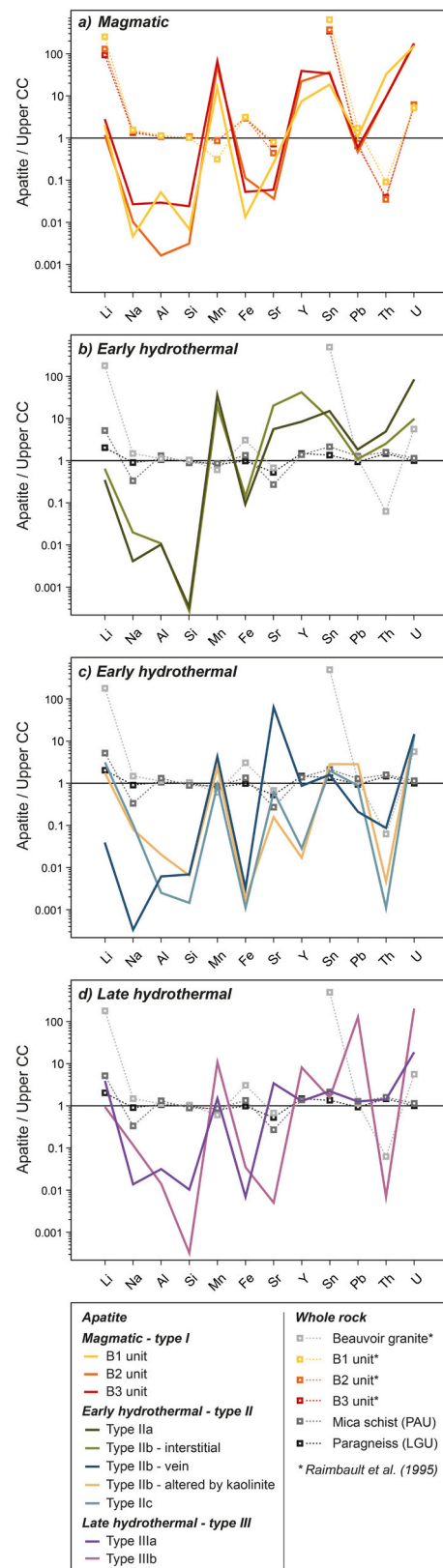
Fig. 8. Trace elements distribution normalised to the upper continental crust (CC) (Rudnick and Gao, 2003) for the distinct apatite generations and the Beauvoir PRMG. Whole rock trace elements distributions for the Beauvoir granite (Raimbault et al., 1995), the Sioule mica schist and paragneiss (Table S9 in Supplementary Material 2) are plotted as references. PAU: Parautochthonous Unit; LGU: Lower Gneiss Unit.
