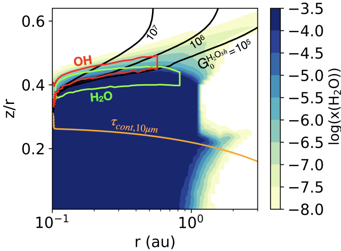
Fig. 3. Disk thermochemical structure of our fiducial model. The emitting area of the rotationally excited OH line at 10.07 \mu\text{m} and the \text{H}_2\text{O} line at 12.519 \mu\text{m} are overlaid on the distribution of the gas-phase water abundance in the disk (color map) and the local FUV radiation field attenuated by gas and dust (black contours) for our fiducial model.
