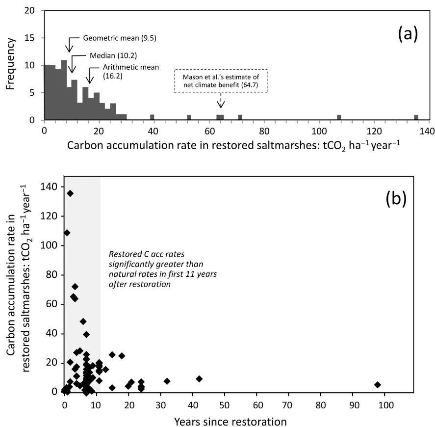
FIGURE 1 | Additional analyses of the global data set of carbon accumulation rates for restored salt marshes expressed as t\text{CO}_2\text{ ha}^{-1}\text{year}^{-1} from the Mason et al. (2023) database. (a) Frequency distribution showing strong skewness (kurtosis), with range of values for their central tendency. Mason et al.'s estimate of net climate benefit also shown, after correcting for \text{CH}_4 and \text{N}_2\text{O} fluxes. (b) Carbon accumulation rates as a function of time since restoration, showing that high initial rates are not sustained.
