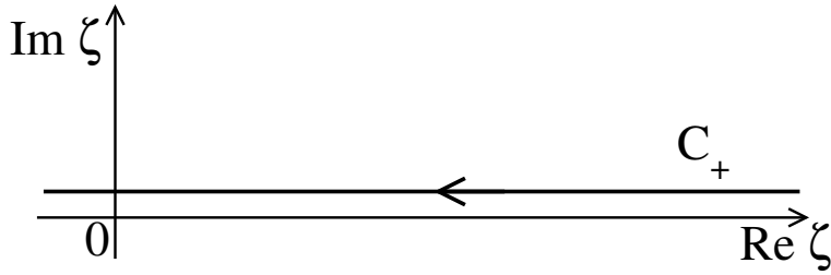
Figure 7. Integration path in the complex plane followed by equation (47).
