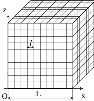
Figure 6. Cutting the gas into mesoscopic cubic portions of side \ell , in the quantum hydrodynamics of Landau and Khalatnikov (this effective theory does not describe length scales < \ell ). See text for choice of \ell .
