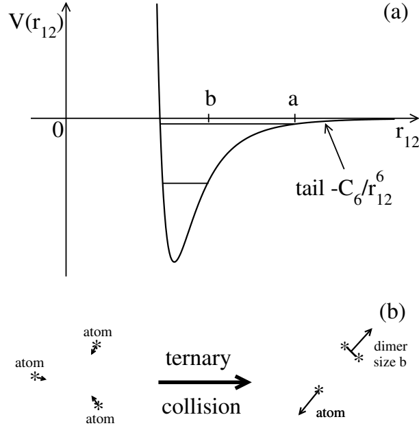
Figure 1. (a) Schematic representation of the resonant van der Waals interaction ( |a| \gg b ) between \uparrow and \downarrow fermions. The potential supports at least one strongly bound state of extension of the order of the van der Waals length b \simeq (mC_6/\hbar^2) and therefore of binding energy \simeq \hbar^2/mb^2 and, in the case of a scattering length a > 0 as in the figure, a last energy level of extension a (of binding energy \hbar^2/ma^2 ) on “the verge of disappearing”; if a were large but negative ( |a| \gg b, a < 0 ), this weakly bound state would be on “the verge of appearing”. (b) The strongly bound dimer state can be populated by three-body collisions and is at the origin of particle losses in the Fermi gas, known as three-body losses. The arrows represent the linear momenta before and after the collision.
