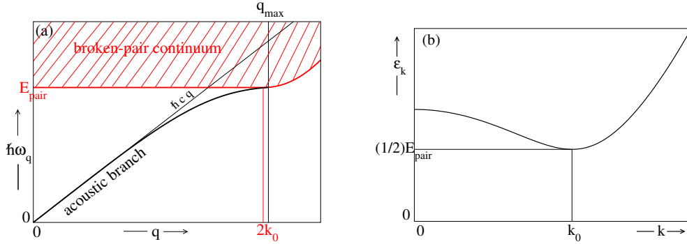
Figure 5. Energy of different types of excitation of an unpolarized homogeneous two-component Fermi gas at zero temperature, as a function of its wave number q or k . (a) Acoustic excitation branch \hbar\omega_{\mathbf{q}} of linear departure \hbar c q ( c is the speed of sound), bounded at the top by the broken-pair continuum (hatched area). Here, the branch tangentially reaches the lower edge of the continuum at the terminal point of wave number q_{\max} . Under the effect of a percussive excitation of wave vector \mathbf{q} , a bound pair \uparrow\downarrow of the pair condensate, initially at rest, dissociates into two fermionic quasiparticles \gamma of opposite spins (see text), wave vectors \mathbf{k} and \mathbf{k}' = \mathbf{q} - \mathbf{k} and energies \varepsilon_{\mathbf{k}} and \varepsilon_{\mathbf{k}'} ; as vector \mathbf{k} is not constrained (no conservation of energy), a continuum of final energies \{\varepsilon_{\mathbf{k}} + \varepsilon_{\mathbf{q}-\mathbf{k}}, \mathbf{k} \in \mathbb{R}^3\} appears. For the interaction strength chosen in the figure ( |\Delta|/\mu = 0.84 or 1/k_{\text{F}}a \simeq -0.16 according to BCS theory, with \mu the chemical potential of the gas and \Delta the complex order parameter of the pair condensate), the acoustic branch is concave at low q ( \gamma < 0 in equation (33)) and (b) the dispersion relation \varepsilon_{\mathbf{k}} has a minimum E_{\text{pair}}/2 at k = k_0 > 0 ; the lower edge of the continuum is therefore exactly E_{\text{pair}} , at least as long as one can have k = k' = k_0 , i.e. as long as q = |\mathbf{k} + \mathbf{k}'| \leq 2k_0 . The approximate dispersion relations shown are derived from BCS theory for \varepsilon_{\mathbf{k}} and Anderson's RPA for \hbar\omega_{\mathbf{q}} . Depending on the interaction strength, the domain of existence in q of the acoustic branch may also be non-compact, connected q \in ]0, +\infty[ or not q \in ]0, q_{\max}[ \cup ]q_{\min}, +\infty[ ( q_{\min} > q_{\max} ) [42]; the concavity of the branch is also variable [43]; finally, k_0 = 0 and E_{\text{pair}} = 2(\mu^2 + |\Delta|^2)^{1/2} if \mu < 0 , k_0 = (2m\mu)^{1/2}/\hbar and E_{\text{pair}} = 2|\Delta| otherwise.
