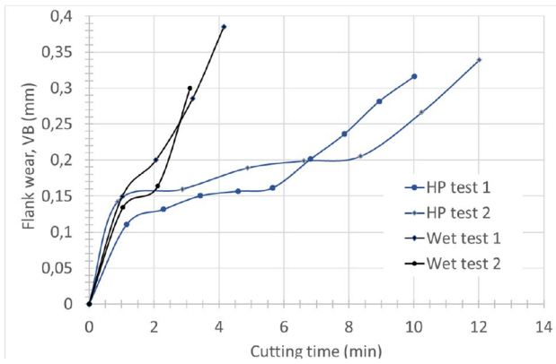
Fig. 17 Evolution of flank wear as a function of time for tests with and without HPA
