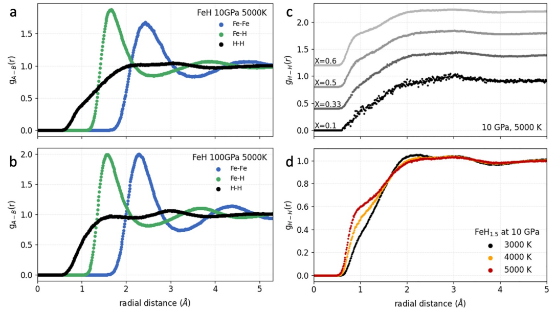
Figure 2. Typical pair distribution functions ( g_{A-B}(r) ) of the bonds in the iron hydride melts, shown at 5,000 K and P_{\text{NSP}} = 10 GPa (a) and 100 GPa (b) for \text{Fe}_{0.5}\text{H}_{0.5} . The g_{\text{Fe-Fe}}(r) and g_{\text{Fe-H}}(r) follow a structure typical of melts with a pronounced first peak and trough. By contrast, the g_{\text{H-H}}(r) is flat with values around 1: the probability of finding a hydrogen a certain distance from another is approximately equal. At 100 GPa, the g_{\text{H-H}}(r) increases more quickly to g_{\text{H-H}}(r) = 1 ; hydrogen is more likely to be further from itself at low pressure. The 10 GPa g_{\text{H-H}}(r) at 5,000 K for each composition lifted from the y-axis for ease of comparison (c). A peak at around 1 Å develops as the hydrogen concentration increases, indicating increased amounts of molecular hydrogen. The g_{\text{H-H}}(r) in \text{Fe}_{0.4}\text{H}_{0.6} at 3,000, 4,000, and 5,000 K (d). The molecular peak gains strength as temperature increases.
