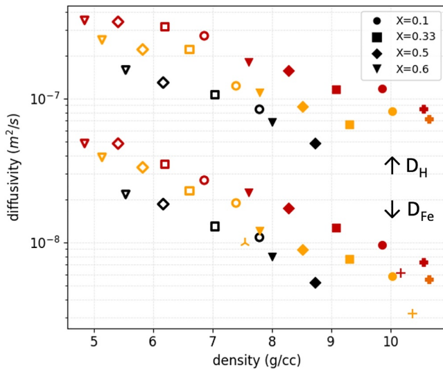
Figure 8. The diffusivities of iron and hydrogen in the P_{\text{NSP}} = 10 (hollow symbols) and 100 GPa (filled symbols) melts as a function of density (black: 3,000 K, gold: 4,000 K, scarlet: 5,000 K). Also shown is the diffusivity of pure iron from Zhang et al. (2000) (thin crosses) and Li and Caracas (2021) (triangle cross) and of hydrogen and iron in \text{Fe}_{0.91}\text{H}_{0.09} from Li et al. (2022) (thick crosses). Pressure suppresses diffusion, while temperature enhances it. Hydrogen is more diffusive than iron. As the melts become more hydrogen-rich (density decreases), the diffusivity of both iron and hydrogen generally increases. The diffusivity of the iron changes at a faster rate with density than that of hydrogen: the diffusivity of iron is more sensitive to hydrogen concentration.
