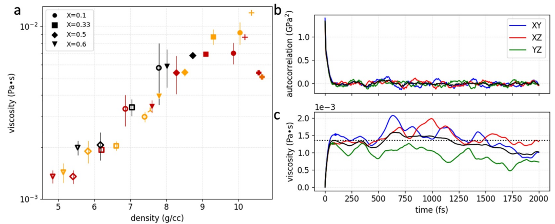
Figure 9. Shear viscosity of the iron hydrides (a) in the P_{\text{NSP}} = 10 (hollow symbols) and 100 GPa (filled symbols) melts as a function of density (black: 3,000 K, gold: 4,000 K, scarlet: 5,000 K). The melts are less viscous at higher temperature and more viscous at higher pressure. More hydrogen-rich (less dense) melts are generally less viscous than the other melts at the same pressure and temperature. For comparison, the viscosity of pure iron from Zhang et al. (2000) (thin crosses) and Li and Caracas (2021) (triangle cross) and of \text{Fe}_{0.91}\text{H}_{0.09} from Li et al. (2022) (thick crosses). Representative stress autocorrelation functions (b) and shear viscosity (c) for the shear components of the stress tensor \sigma_{ij} , i \neq j , as functions of time window for \text{Fe}_{0.5}\text{H}_{0.5} at P_{\text{NSP}} = 10 GPa and 5,000 K. The black curve represents the average of the results from each component of the stress tensor. The stress autocorrelation drops to zero after 100 steps. The value of the viscosity reaches convergence shortly after. The differences between shear tensor components are normal numerical effects and give a sense of the error bars in our viscosity estimates. For consistency with previous studies, we plot in (a) the viscosity values obtained when the average of the autocorrelation functions first cross zero (Zhang et al., 2000).
