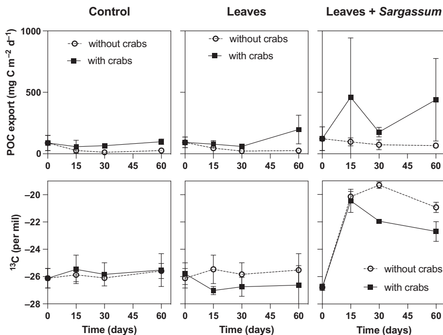
Fig. 3. Top: evolution of particulate OC export by the simulated tide ( \text{mg C m}^{-2}\text{d}^{-1} ) and bottom: temporal dynamic of \delta^{13}\text{C} signature of POM in the three experimental treatments (control, L, and L + S). Error bars are standard deviations from the mean of three tanks (treatment + absence/presence of crabs) and six tanks at T0, before the contribution of crabs. L, leaves; L + S, leaves + Sargassum ; OC, organic carbon; POM, particulate organic matter.
