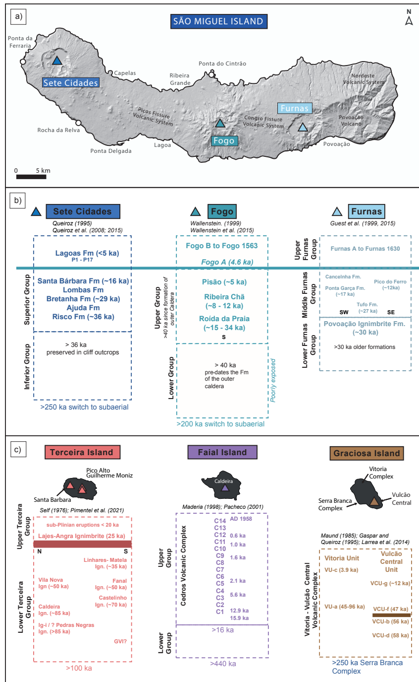
Figure 3: (a) Map of São Miguel and the location of the three trachytic central volcanoes Sete Cidades, Fogo and Furnas (Basemap: NASA JPL; 2021). Simplified volcanostratigraphic scheme for (b) São Miguel, and (c) Terceira, Faial and Graciosa's volcanoes. These are based on those presented by Queiroz (1997), Queiroz et al. (2008; 2015), Wallenstein (1999), Wallenstein et al. (2015); Guest et al. (1999; 2015); Self (1976); Gertisser et al. (2010), Pimentel et al. (2021), Maderia (1998), Pacheco (2001); Maund (1985), Gaspar (1996), Larrea et al. (2014), respectively.
