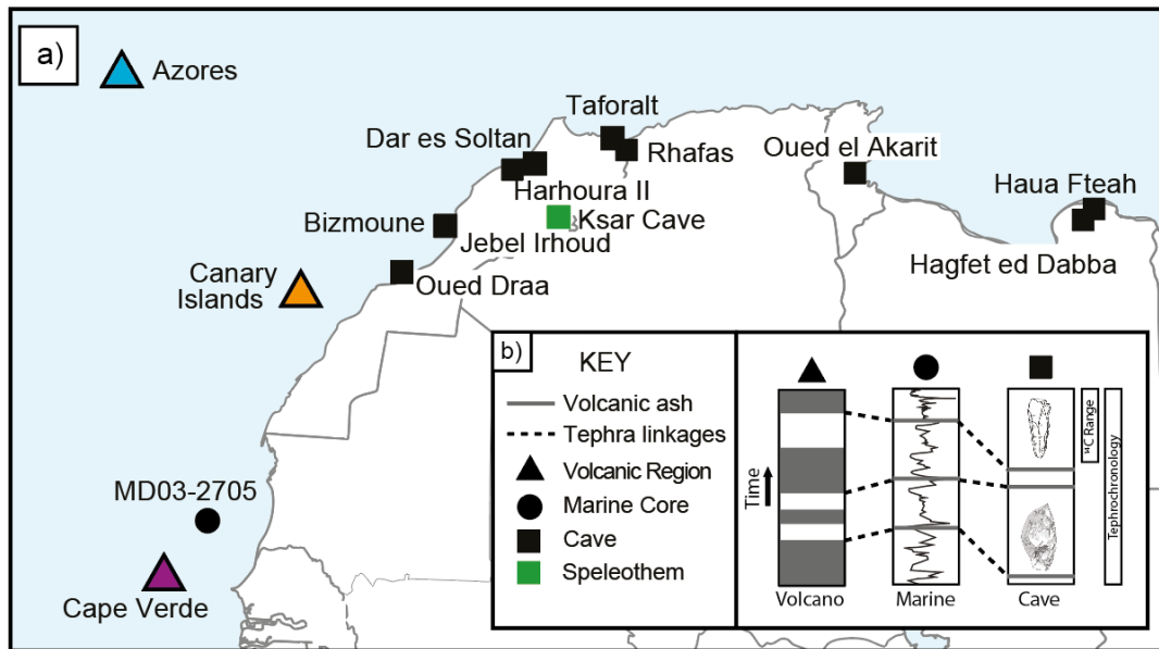
Figure 1: (a) Location of key MSA-LSA archaeological and climate records (e.g., MD03-2705; Skonieczny et al., 2019) in North West Africa and the key volcanic source regions of greatest relevance for this region. (b) Schematic showing the potential of identifying co-located volcanic ash (tephra) layers. These time-parallel markers permit possibilities to: (i) share chronological information and (ii) directly compare climatic and cultural changes.
