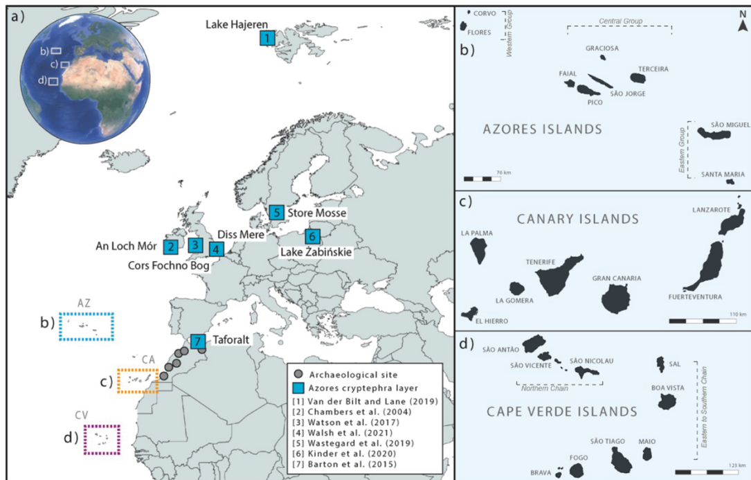
Figure 2: (a) Location of the key volcanic regions located within the North Atlantic, including the islands of the (b) Azores (AZ), (c) Canaries (CA), and (d) Cape Verde (CV), of greatest relevance for ash dispersal across NW Africa. The distal sedimentary palaeoenvironmental records reported to contain volcanic ash erupted from the Azores are marked with a blue box (Chambers et al., 2004; Barton et al., 2015; Watson et al., 2017; van der Bilt and Lane, 2019; Wastegård et al., 2020; Kinder et al., 2020; Walsh et al., 2021).
