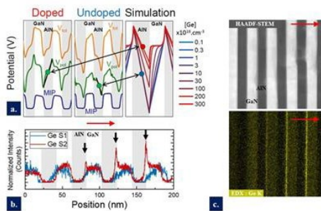
Fig.2: The red arrow represents the [0001] growth direction. [a] Comparison of the potential profiles for the doped (S2) and undoped (S1) potential with simulations (nextnano3 software), showing an inversion of the electric field in the AlN layer for the doped sample. [b] EDX profile of the germanium for S1 and S2. The signal observed for S1 is an artefact due to the proximity of K \alpha energy band for Ga and Ge. The black arrows highlight the Ge peak at AlN/GaN interfaces. [c] HAADF-STEM image of the AlN/GaN superlattice and EDX map of the Ge, showing the accumulation of Ge at interfaces.
