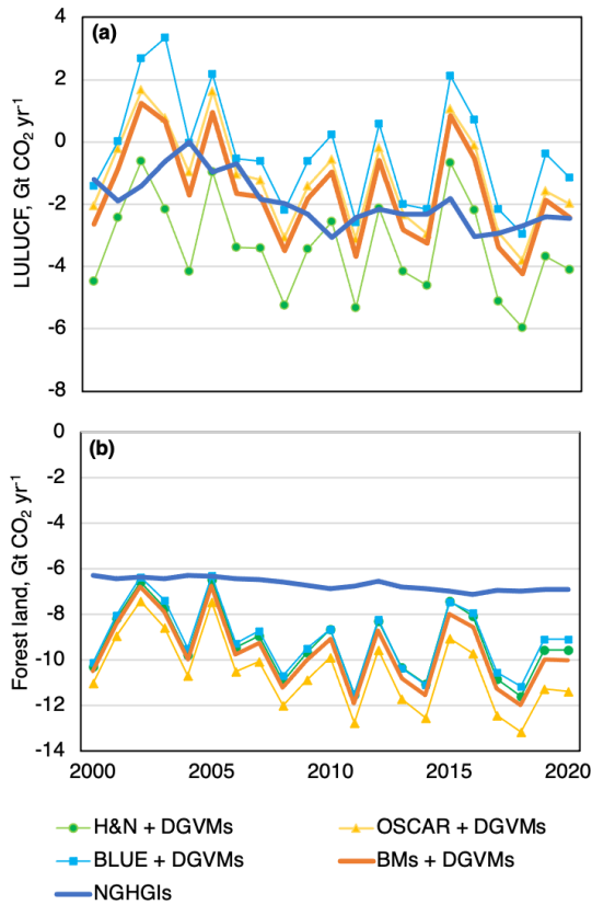
Figure 6. Adjusted CO 2 fluxes from BMIs for LULUCF (panel a) and for forest land (b), i.e. original BMIs' results plus the natural sink from DGVMs in non-intact forest, compared to the NGHIGs for the period 2000–2020.
