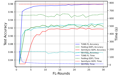
(b) CIC-IDS2017
