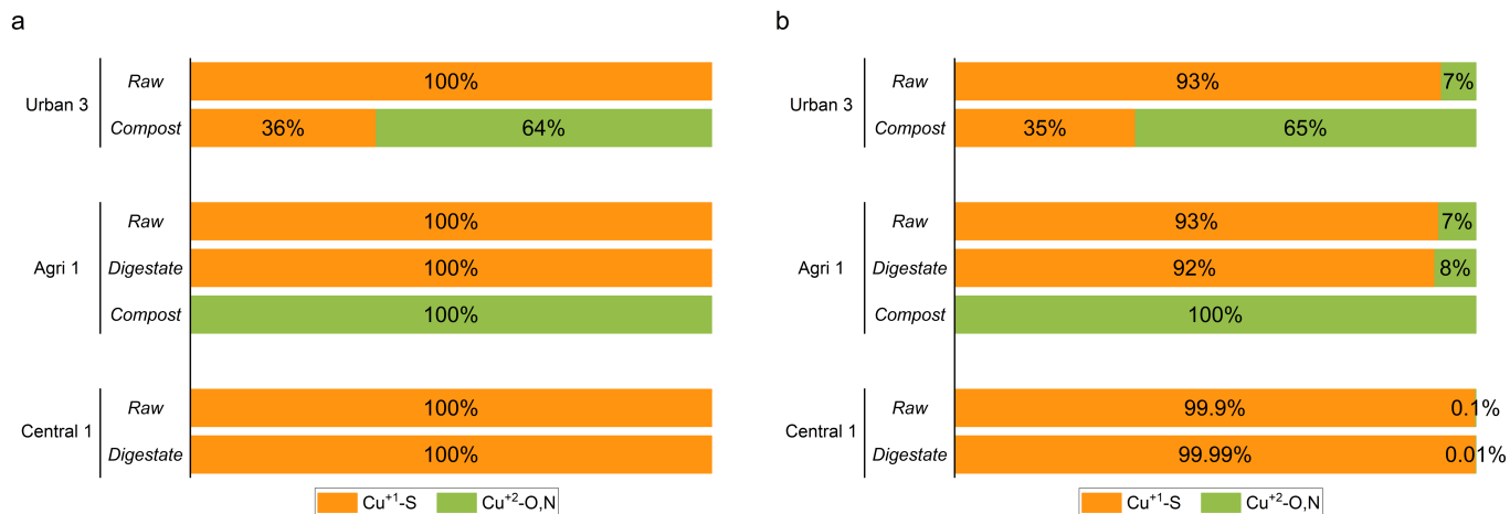
Figure 4: Comparison of Cu speciation of raw and treated OWs determined from the LCF of (a) the standard bulk Cu K-edge XANES spectra and (b) the cluster spectra derived from the PCA and cluster analyses of the Cu K-edge XANES map.
