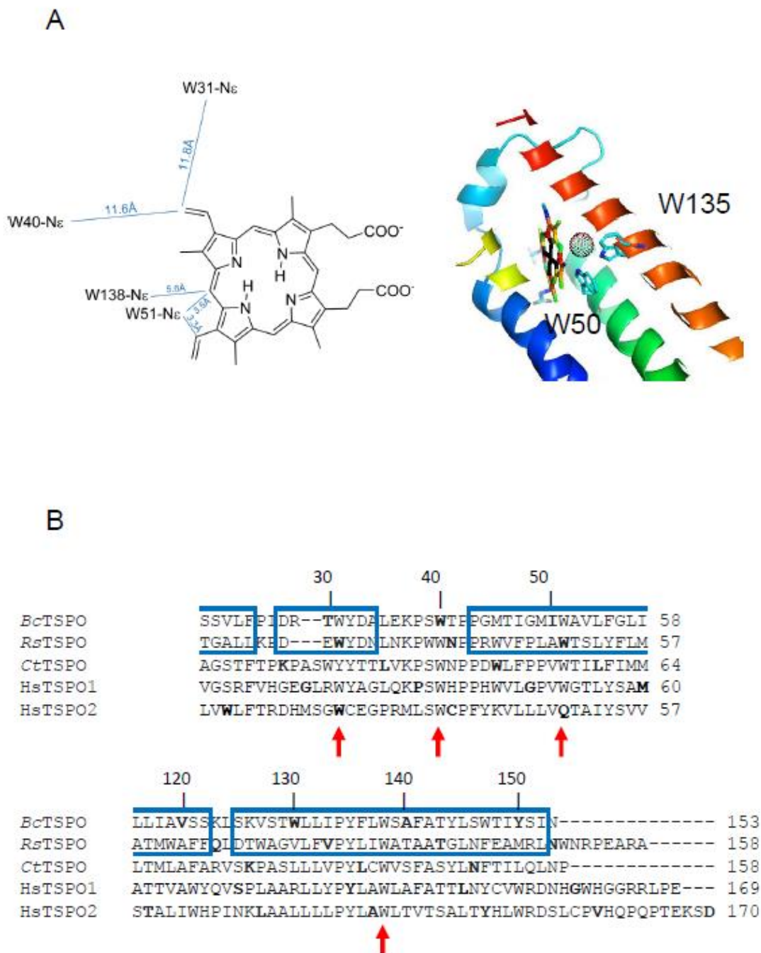
Figure 9: (A) Left, Potential amino acids involved in the binding and catalysis of PPIX by Bc TSPO (adapted from [6]). Right, inside view of heme in Rs TSPO (PDB code 8E7W). W50-N \epsilon and W135-N \epsilon of Rs TSPO are located to the closest CH Meso of heme at 3.5 and 5.9 Å, respectively and closest vinyl at 5.2 and 6.7 Å, respectively; among the various water molecules present in the binding cavity, the closest one is at ~6 Å of heme on the same side of W50 and W135 side chain. (B) Amino acid sequence alignment given in one-letter code and identified by species abbreviations: Bc , Bacillus cereus ; Rs , Rhodobacter sphaeroides ; Ct , Chlorobium tepidum ; Hs , Homo sapiens . Bold amino acids correspond to tenth within the sequence. Blue boxes correspond to helical structures of transmembrane domains or loop.
