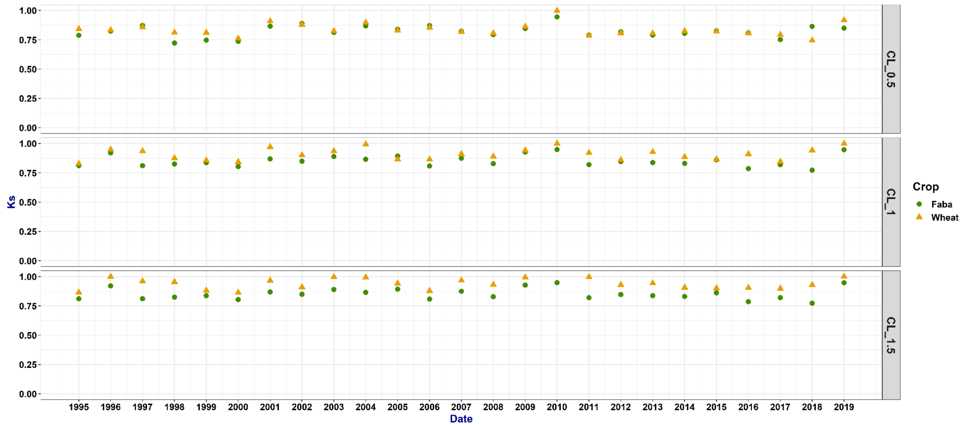
124 Fig. SF5 (part 2/3): Mean water stress coefficient (Ks), calculated for faba bean (green disks) and wheat (yellow triangles) when considering simulations without connectivity. 125 A Ks equal to 1 corresponds to no water stress, while a Ks equal to 0 corresponds to full water stress. CL represents Clay-Loam texture, respectively. The labels “_0.5”, “_1”, 126 and “_1.5” denote soil depths of 0.5 m, 1 m, and 1.5 m, respectively.
