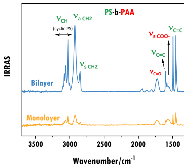
Figure 8. PM-IRRAS spectra of a \text{PS}_{394}\text{-}b\text{-PAA}_{58} mono- and bilayer.
