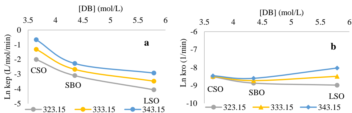
Fig. 13. Kinetic comparison of \text{Ln } k_{ep} and \text{Ln } k_{ro} versus the initial double bond concentration for the epoxidation of vegetable oils at different temperatures. ( \text{Ln } k_{ep} : The natural logarithm of rate constants for epoxidation; \text{Ln } k_{ro} : The natural logarithm of rate constants for ring-opening)
