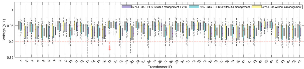
Fig. 13. The voltage levels for LV transformers with and without LCTs.
