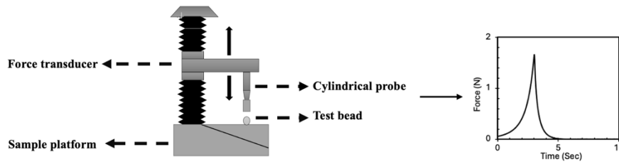
23 24 Fig. 2 Schematic illustration of compression tests of PVA-ALG bead
