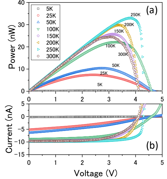
Fig. 3. (a) P - V and (b) I - V characteristics of diamond pn junction diodes at 5 K to 300 K.
