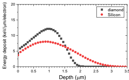
Fig. 2. Depth profile of the electron beam energy deposit
