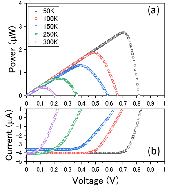
Fig. 4. (a) P - V and (b) I - V characteristics of Si-PiN diode from 50 K to 300 K.
