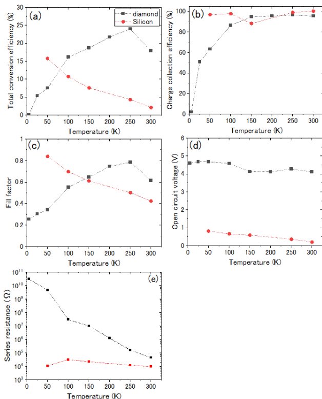
Fig. 5. Betavoltaic parameters of diamond pn and Si-PiN diodes with various temperature. (a) Total conversion efficiency( \eta ), (b) Charge collection efficiency( Q ), (c) Fill factor( FF ), (d) open circuit voltage( V_{oc} ), and (e) series resistance( R_s ).
