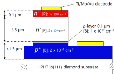
Fig. 1. Schematic of the pseudo vertical diamond pn junction diode
