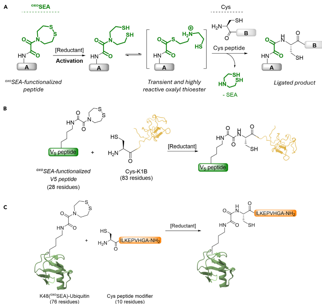
Figure 1. The chemistry of oxalyl thioester precursors
