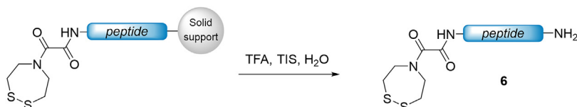
Figure 7. Synthetic approach for the preparation of an N-ter functionalized V5 tag-derived peptide with an ^{\text{oxo}} SEA handle
