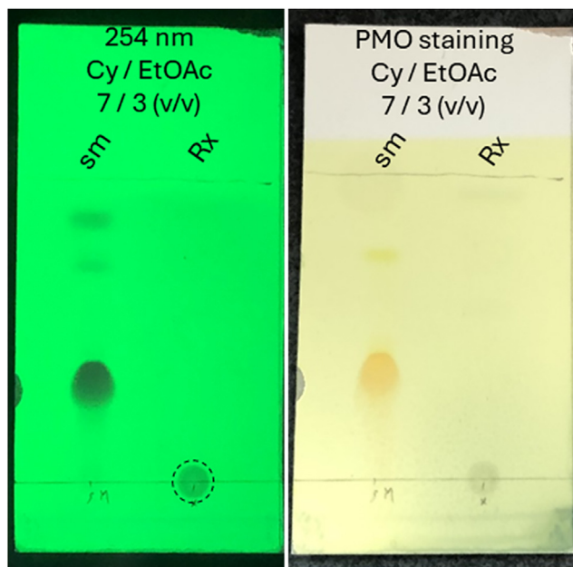
Figure 6. TLC-monitoring of the reaction (Sm = Starting material; Rx = crude reaction mixture) Reaction completion is indicated by disappearance of the starting material spot ( R_f = 0.32 ).
