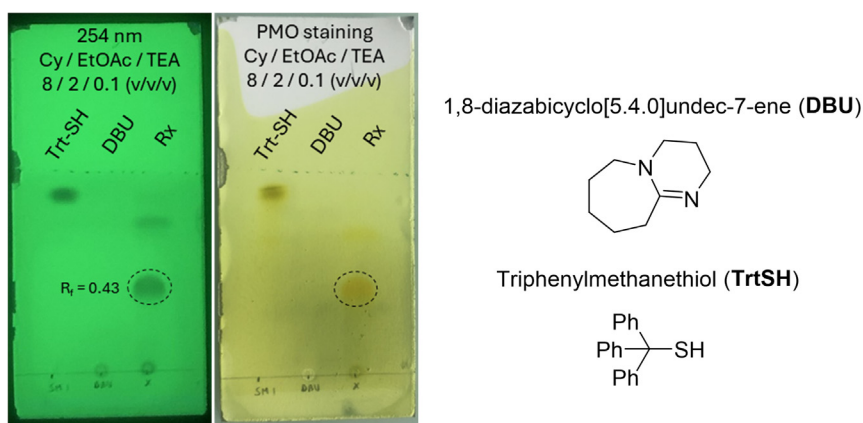
Figure 2. TLC-monitoring of the reaction
