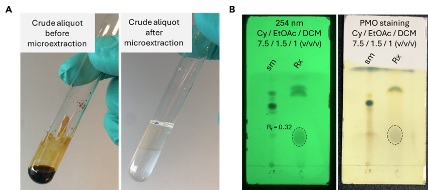
Figure 5. Monitoring of iodine-mediated trityl group cleavage
