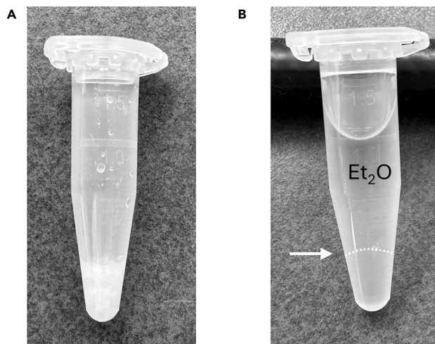
Figure 13. Extraction of MPAA before HPLC-analysis
