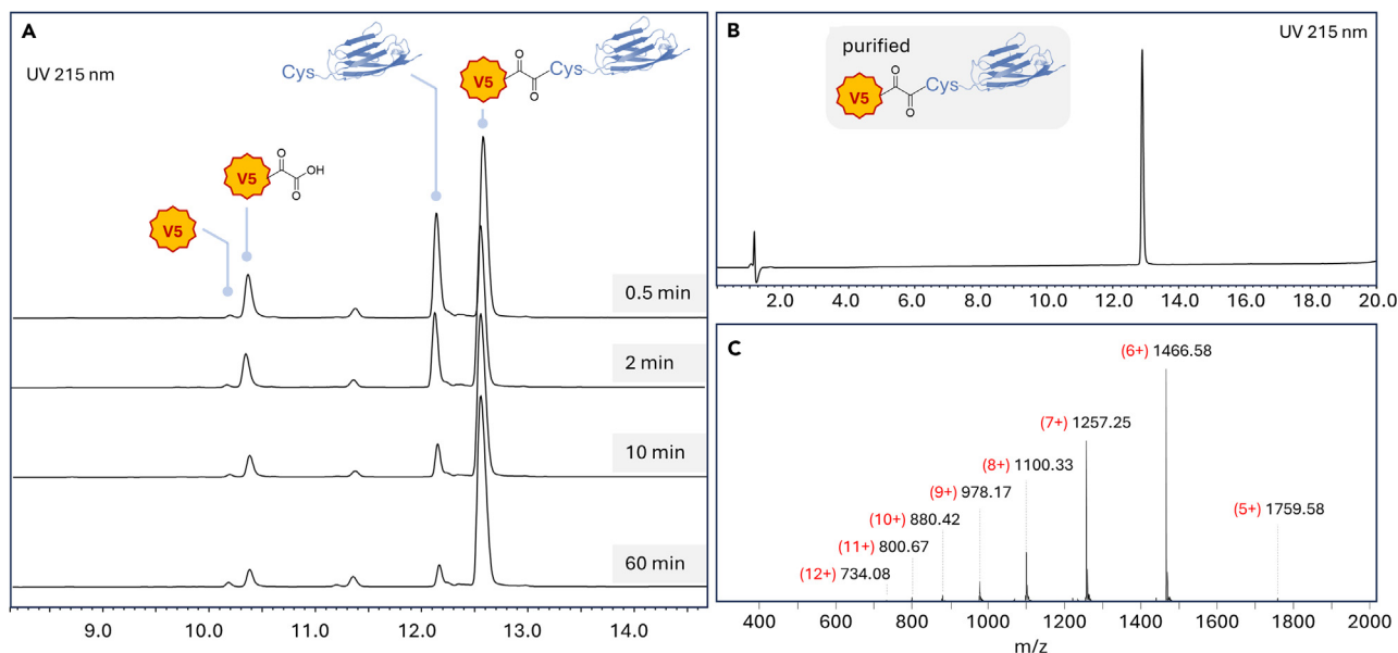
Figure 11. Synthesis of the V5-oxo-Cys-GSGS-GB1 conjugate
