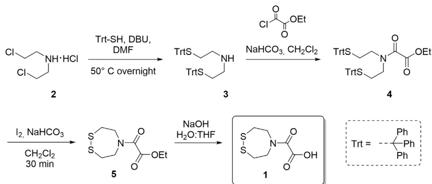
Scheme 1. Synthetic approach towards 99 SEA handle 1
