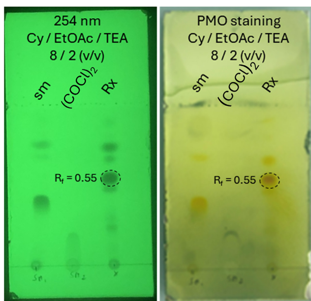
Figure 4. TLC-monitoring of the reaction (Sm = starting material; Rx = crude reaction mixture) The expected product corresponds to the spot at R_f = 0.55 .
