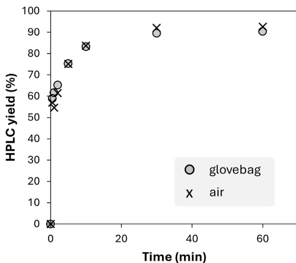
Figure 12. Kinetic monitoring of the \text{oxoSEA} -mediated ligation reactions between peptide 6 and Cys-GSGS-GB1 conducted in a glovebag (gray circles) or on the bench (black crosses)
