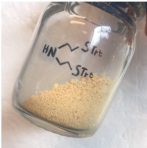
Figure 3. Bis(2-(triphenylmethylthio)ethyl)amine 3 is obtained as a yellowish powdery solid
