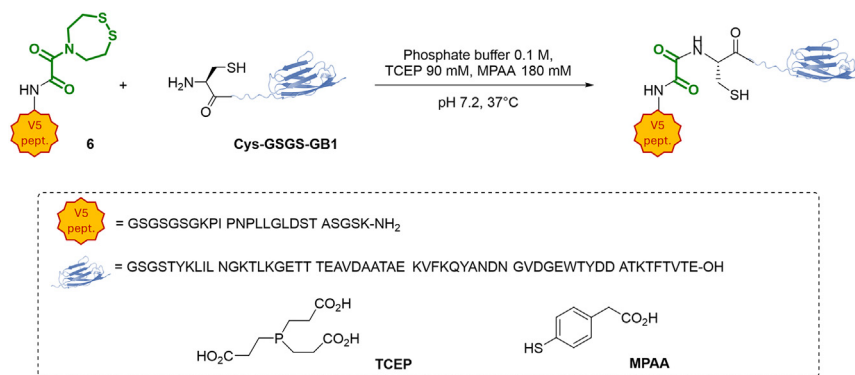
Figure 9. oxo SEA-mediated ligation of V5 peptide 6 with Cys-GSGS-GB1 protein
