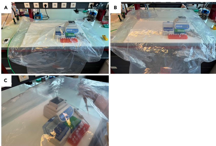
Figure 10. Glovebag installation and preparation
