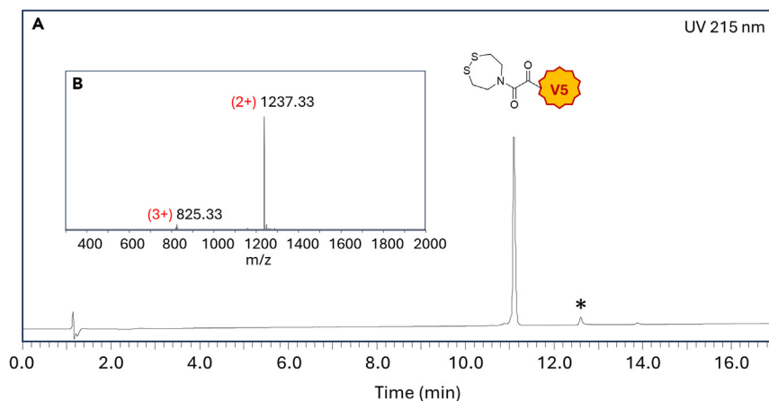
Figure 8. Analysis of purified V5- oxo SEA peptide 6
