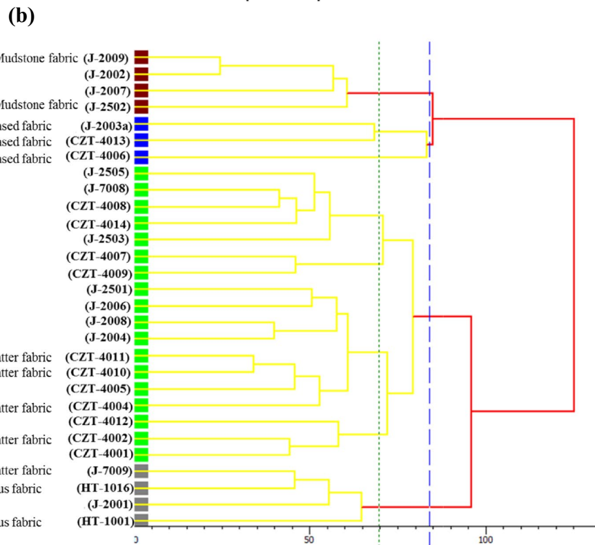
Fig. 3 a PCA plot of ceramic bodies (73.87% var) based on XRPD diffractograms, b Dendrogram of PCA results derived from XRPD diffractograms
