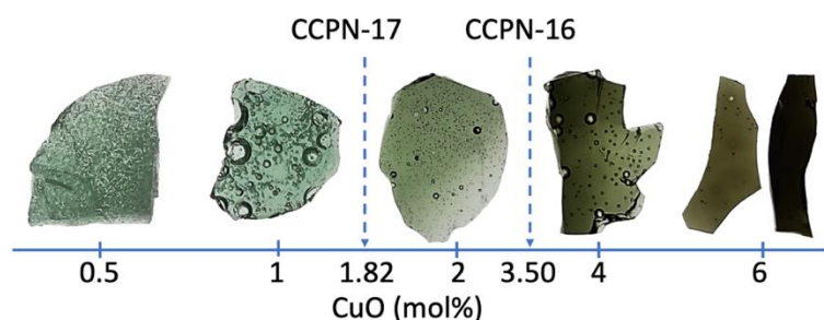
Figure 3. Picture of the glasses of the SiAlCu x series as a function of the CuO mol% and the CCPN-16 and CCPN-17 glazes used at the Manufacture of Sèvres. The last picture shows the most concentrated glass with two thicknesses (330 μm and 1 mm) to highlight the color and the reduced transparency of the highly concentrated glasses.
