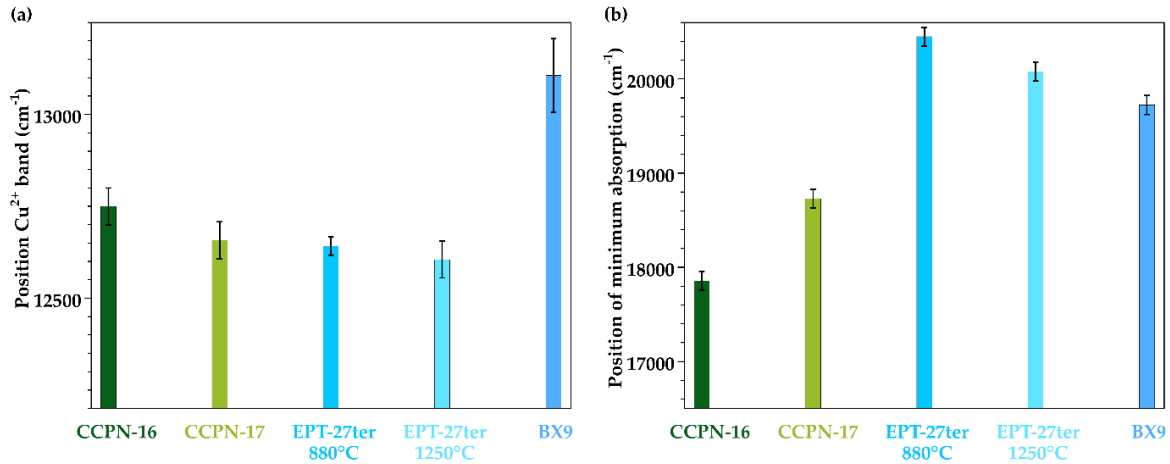
Figure 6. (a) Position of the \text{Cu}^{2+} band. (b) Position of the minimum absorption defining the highest transmission.
