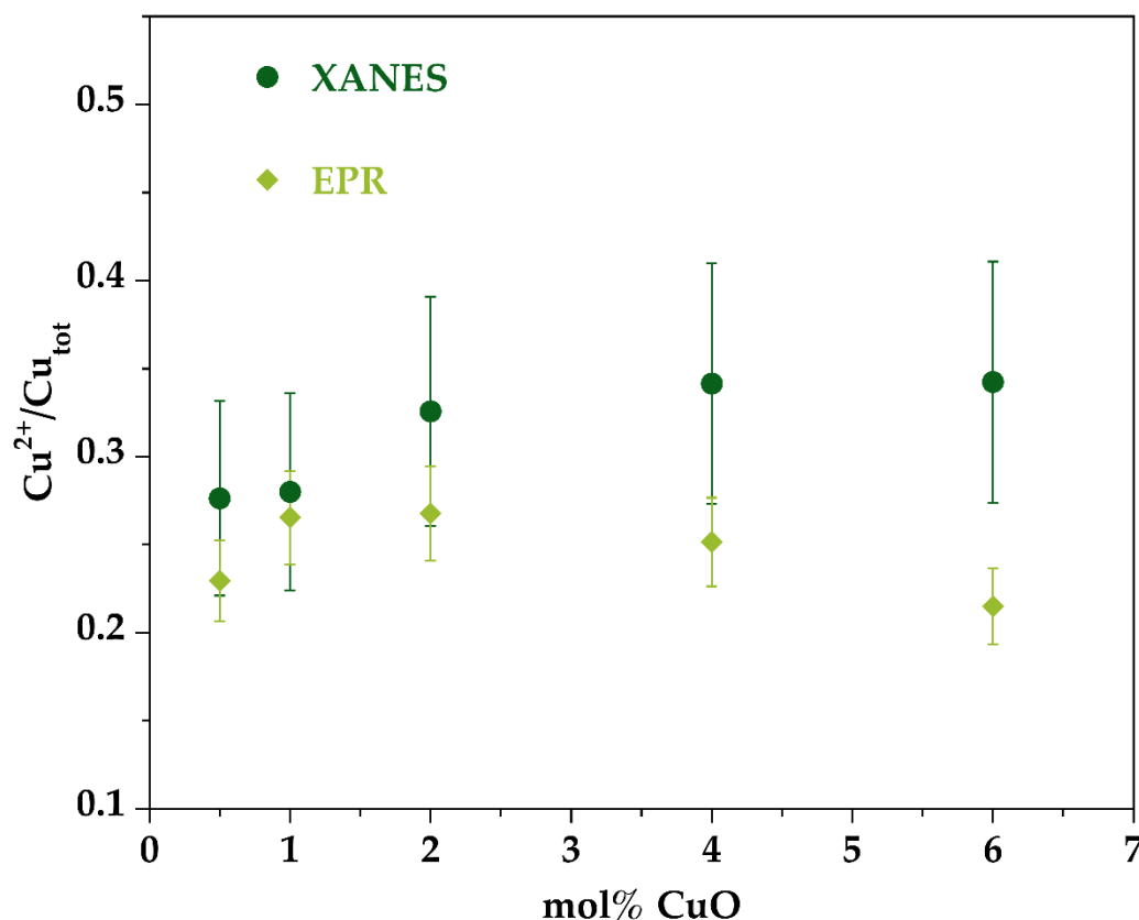
Figure 11. Comparison between the redox ratios determined by EPR and XANES for the \text{SiAlCu}_x glass series.
