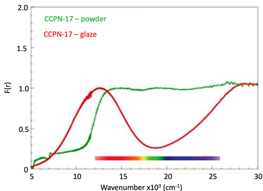
Figure S7. Optical absorption spectra for CCPN-17: initial powder (green) and the glaze applied on the ceramic (red).
