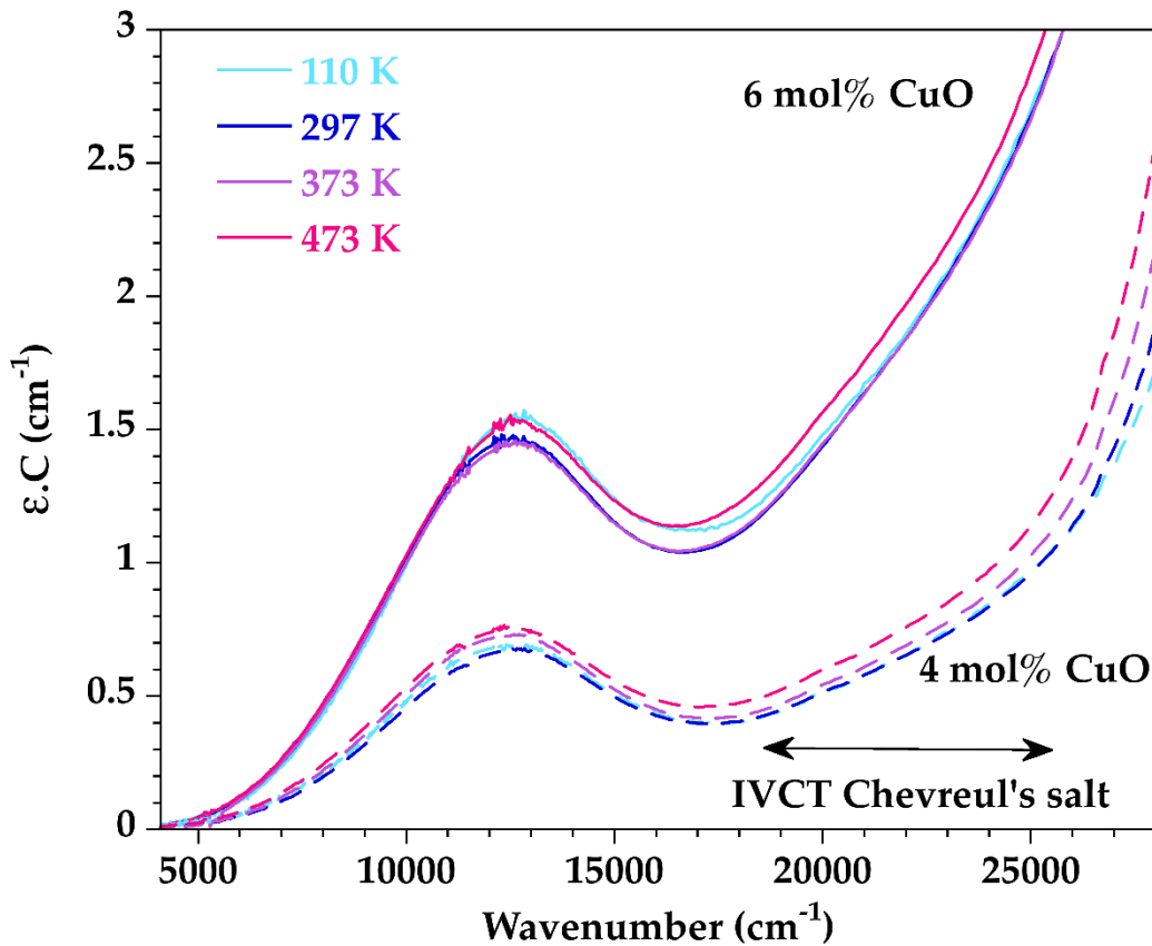
Figure 12. Variation with temperature of the optical absorption spectra for \text{SiAlCu}_x glasses with x = 4 and 6 mol% CuO. The horizontal arrow indicates the region in which IVCT is observed in Chevreur's salt [38], [39].
