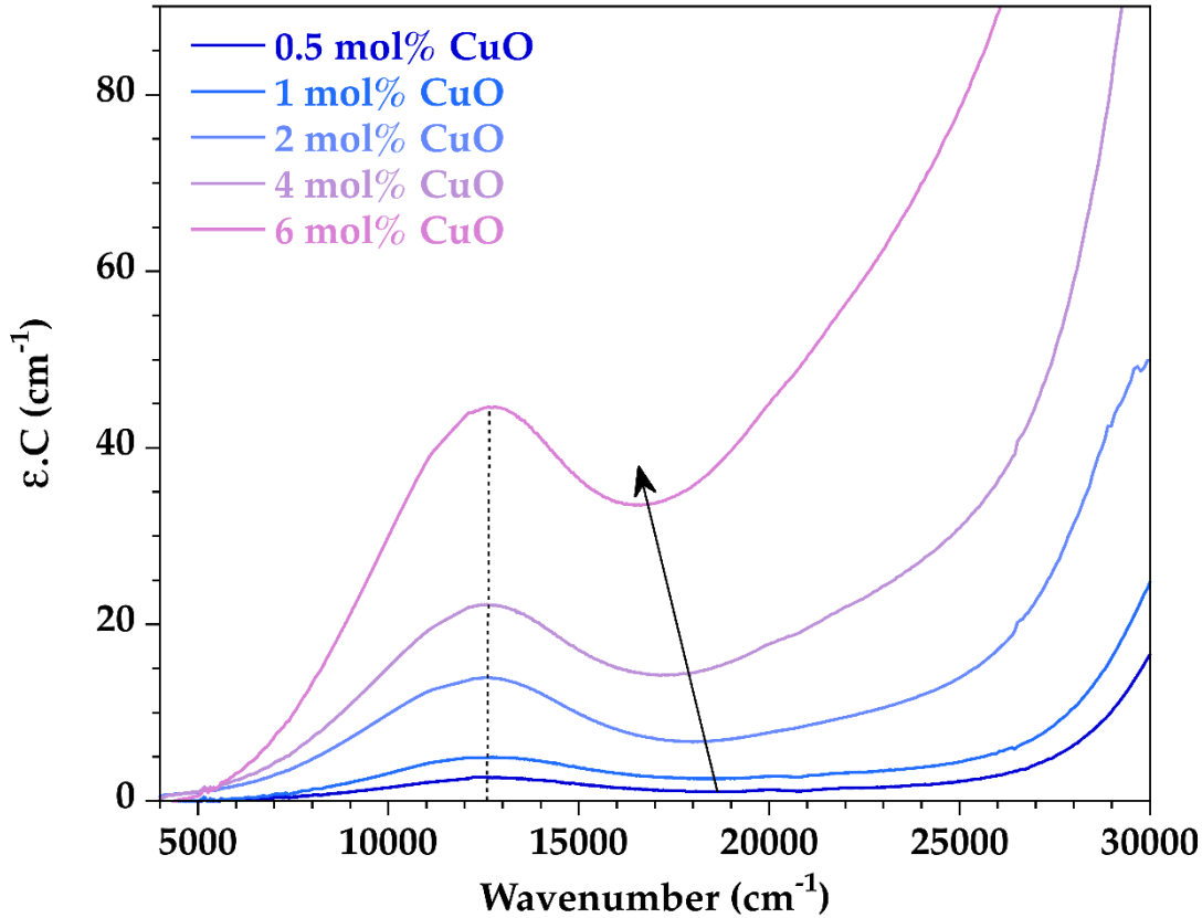
Figure 8. Optical absorption spectra in transmission for the SiAlCu x series.
