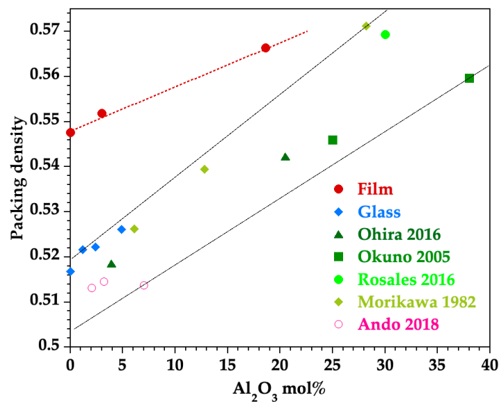
FIGURE S8 Packing density of \text{SiO}_2\text{-Al}_2\text{O}_3 thin films and glasses
