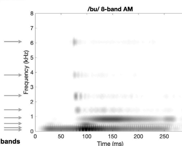
FIGURE 1 The upper panels depict the waveform (left) and spectrogram (right) of one of the French words ( bout /bu/) used in experiments 1 and 2, in intact speech. Its AM and a sample of its FM are depicted in the waveform (orange line and blue box, respectively). The lower panels depict the spectrograms of the vocoded stimuli used in experiments 1 and 2. The grey arrows depict the number of spectral bands in which AM information was preserved, either 16 (left) or 8 (right).
