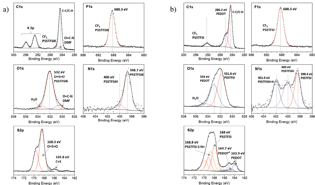
Figure 1. C1s, F1s, O1s, N1s, and S2p XPS spectra and their desummutation for a) PSSTFSIK and b) PEDOT:PSSTFSI.
