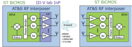
Fig. 5. Transmitter front-end integrating BiCMOS and InP chips within an advanced RF packaging (on the left) and receiver front-end integrating a BiCMOS chip within an advanced RF packaging (on the right).
