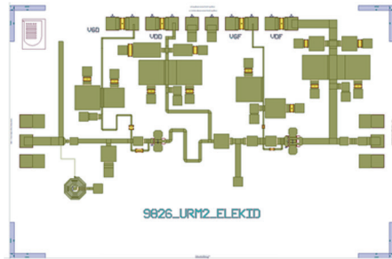
Fig. 3. PA layout. Chip size is 3.0 mm x 2.0 mm.
