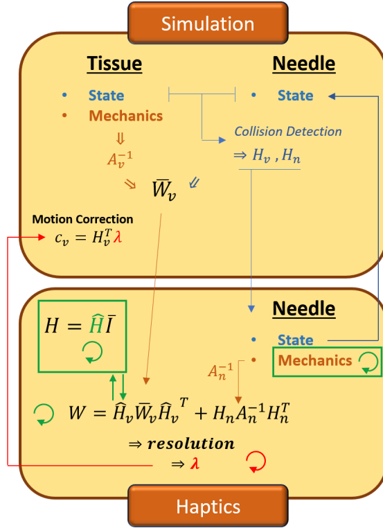
Figure 1: Organization of the simulation and haptic loops, and their communication.
