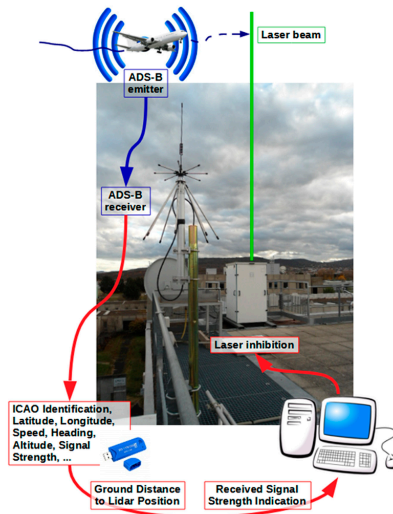
Figure 1. Overview of the air-safety system based on a picture of the outdoor OPGC platform.
