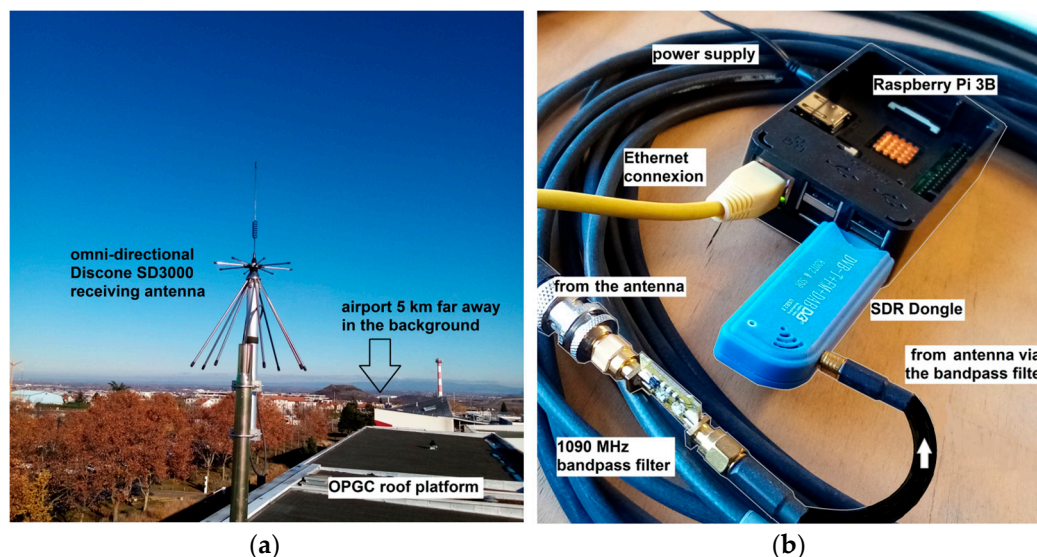
Figure 2. General view of the outdoor (a) and indoor (b) hardware with SDR Dongle and Raspberry Pi.
