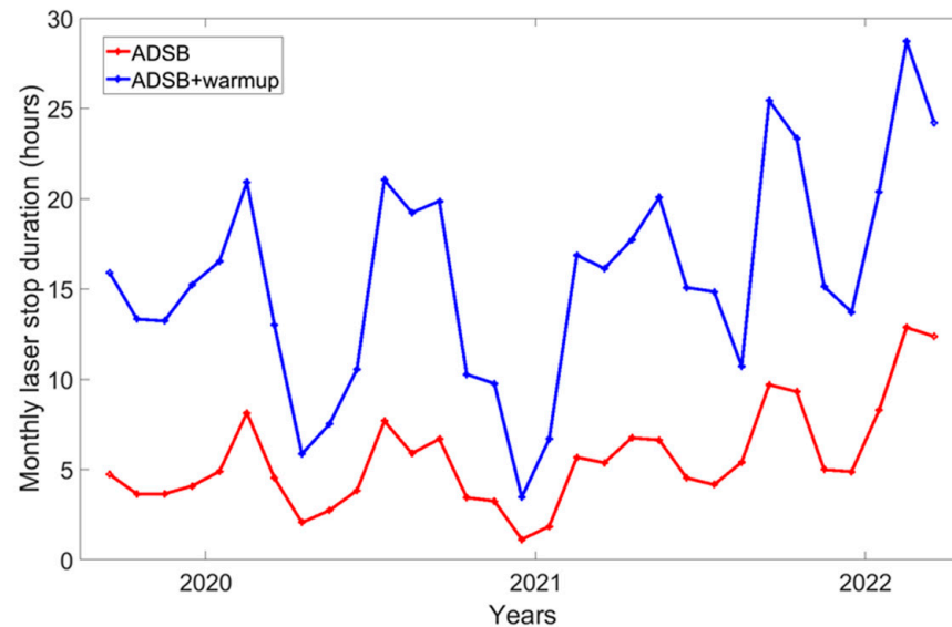
Figure 5. Monthly laser stop and measurement durations. The red line corresponds to the monthly laser stop duration, and the blue line to the measurement stop duration, also including the temporization and warmup time needed to stabilize the laser emission.
