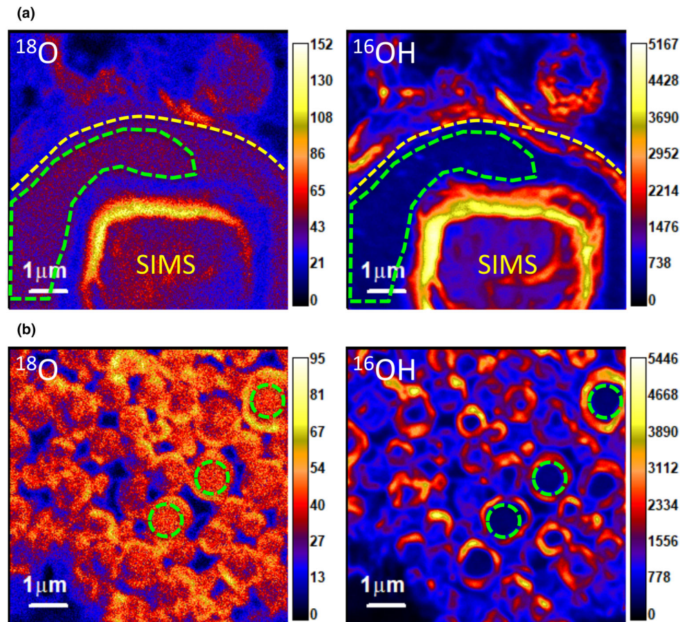
FIGURE 4. Ion images of fibrous magnetite and magnetite microspherules/framboids. (a) Fibrous magnetite 6. The dashed yellow line shows the edge of the grain. (b) Microspherule area in the vicinity (see Figure 1). Green dashed lines: regions of interest selected for data analysis. Ion intensities per pixel correspond to total counts.
