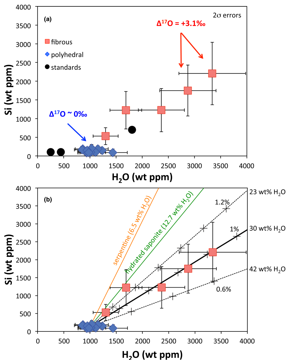
FIGURE 5. (a) Water content as a function of Si content in coarse-grained magnetite from Ryugu. Oxygen isotopic compositions are indicated. The two most water-rich analyses are repeat analyses of mgt grain 6. (b) Graphical representation of mixing calculations to evaluate the H 2 O content of Si-rich nano-inclusions. Plain and dotted lines are mixing lines. Orange and green lines: mixing calculations using CI phyllosilicate compositions. Black lines: mixing calculations using the composition of the most Si-rich amorphous inclusions (type-b) in Dobrică et al. (2023). Numbers on the mixing lines indicate the mixing fraction of Si-rich inclusions. Uncertainties are 2 SDs.
