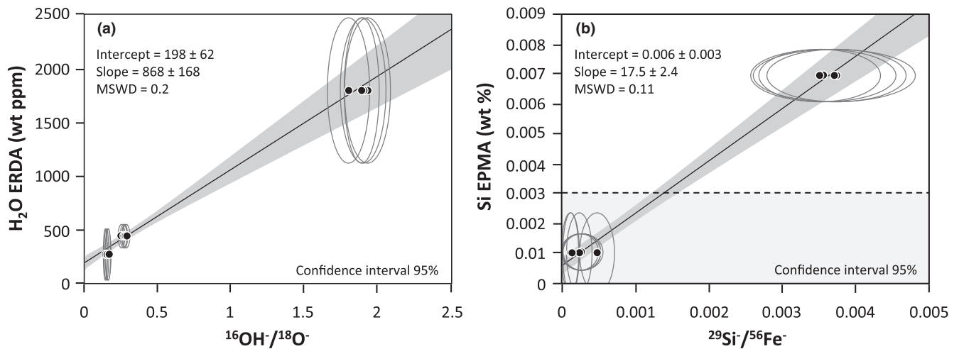
FIGURE 2. Calibrations used for the measurement of water content and Si content in magnetite with the 80 pA beam. (a) Calibration of water content using ERDA. (b) Calibration of Si content using EMPA. The gray area shows the detection limit for EMPA.
