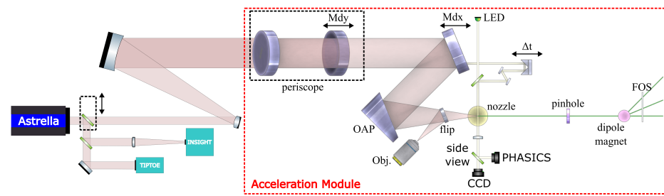
Figure 2. Schematic sketch of the optical setup. The laser beam is sampled by a removable glass wedge to perform the (spatio)temporal characterization using TIPTOE and INSIGHT (not part of the acceleration module). After characterization, the laser beam is expanded by a mirror telescope and coupled into the e-KAIO chamber. The beam is reflected to the upper level by a 45° periscope of mirror Mdy and the upper turning mirror. The mirror Mdx reflects the beam to the off-axis parabola OAP , which focuses the beam into the gas jet above the nozzle. The gas jet is imaged from the top (not displayed) and the side to the respective cameras CCD TopView and CCD SideView (see the GUI in Figure 3) outside the chamber. Additional laser–plasma diagnostics could be added in either arm (outside the vacuum chamber) to investigate the light emitted from the plasma. The flip mirror in between the OAP and the jet can be used to deflect the attenuated beam to microscope objective Obj. , which in turn images the focus onto a camera outside the chamber. The interaction volume can be illuminated from the side either by a continuous white light LED or a small sample beam, extracted from the main beam by a small hole on the side of the mirror Mdx . The quality of the focal spot can be optimized by iteratively adjusting the tip and tilt angles of Mdx and the OAP and the beam pointing is corrected by performing a translational shift before focusing by translating the mirrors Mdy (up/down) and Mdx (left/right). The translational shift leads to a rotation of the laser axis around the focal point and thus can be used to align the laser along the acceleration axis (green). Once aligned, the components of the electron spectrometer ( pinhole , dipole magnet , and FOS ) can be positioned by moving their respective translation stage.
