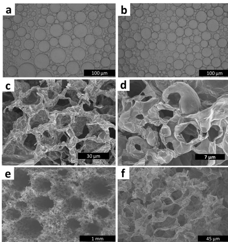
Figure 4. (a, b) Optical microscopy images of Pickering emulsions after addition of methyl polysiloxane resin (a = 38%, b = 23% of functionalized graphene oxide (GO-R16)) and (c, d) Scanning electron microscopy (SEM) images of the porous structure of composites for different formulations (c = 38%, d = 23% of functionalized graphene oxide (GO-R16)) after ceramization, (e, f) Scanning electron microscopy (SEM) images of the porous structure of composites for different formulations (e = 38%, f = 23% functionalized graphene oxide (GO-R16)) in the presence of nickel acetylacetonate after ceramization.
