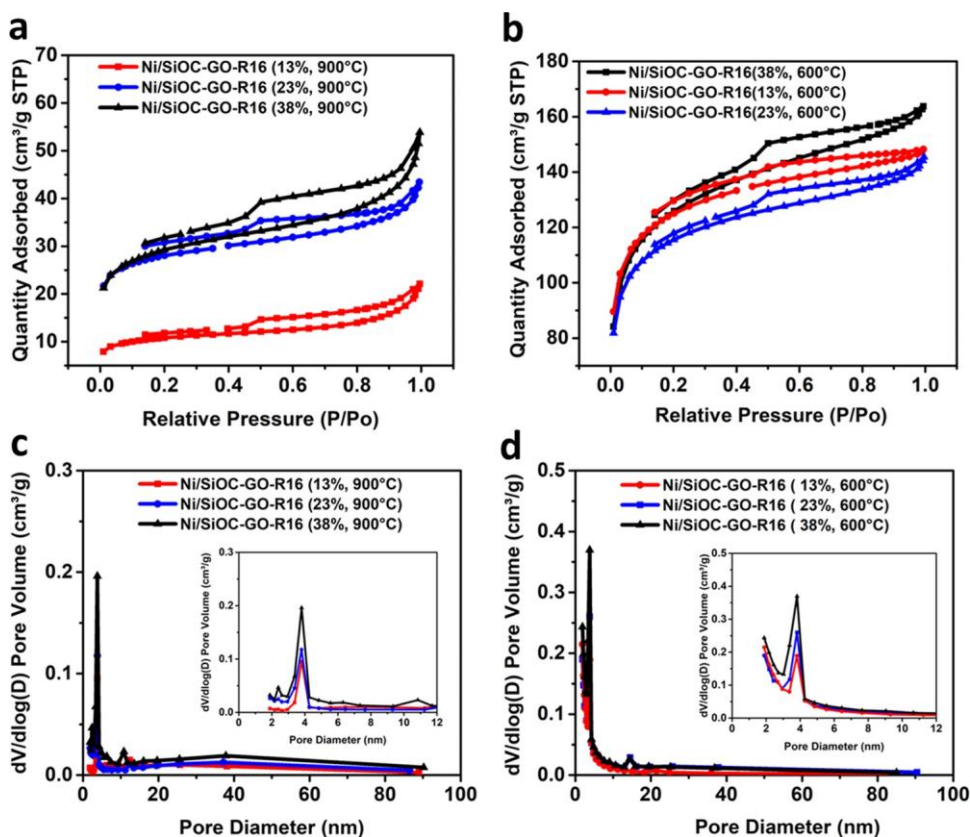
Figure 5. (a, b) N_2 adsorption/desorption isotherms for Ni/SiOC-GO-R16 (X, T ( ^{\circ}C )) composites pyrolyzed at 900 and 600 ^{\circ}C and (c, d) pore size distribution of Ni/SiOC-GO-R16 (X, T ( ^{\circ}C )) composites pyrolyzed at 900 and 600 ^{\circ}C .
