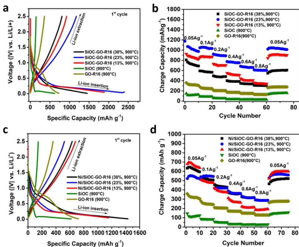
Figure 6. (a) Charge/discharge profile for the 1st cycle at 50 \text{ mA g}^{-1} of composite samples SiOC-GO-R16 ( X, T (^{\circ}\text{C}) ), GO-R16 ( 900 ^{\circ}\text{C} ), and SiOC ( 900 ^{\circ}\text{C} ) pure, (b) cycling performance of composite samples SiOC-GO-R16 ( X, T (^{\circ}\text{C}) ), GO-R16 ( 900 ^{\circ}\text{C} ), and SiOC ( 900 ^{\circ}\text{C} ) pure with increasing current rates, (c) charge/discharge profile for the 1st cycle at 50 \text{ mA g}^{-1} of composite samples Ni/SiOC-GO-R16 ( X, T (^{\circ}\text{C}) ), GO-R16 ( 900 ^{\circ}\text{C} ), and SiOC pure and (d) cycling performance of composite samples Ni/SiOC-GO-R16 ( X, T (^{\circ}\text{C}) ), GO-R16 ( 900 ^{\circ}\text{C} ), and SiOC ( 900 ^{\circ}\text{C} ) pure.
