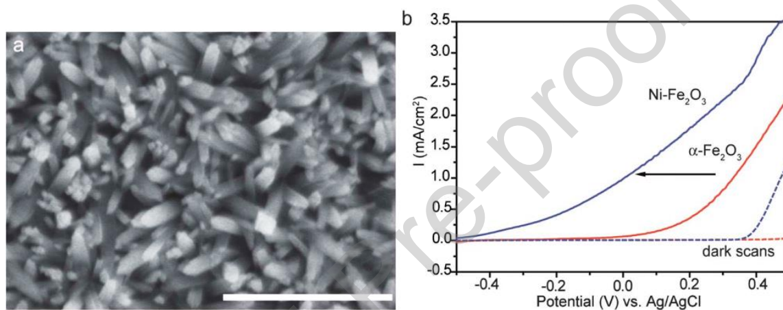
Figure 23. (a) SEM image of an array of \alpha\text{-Fe}_2\text{O}_3 nanowires on FTO; scale bar: 2 \mu\text{m} . (b) Linear scanning voltammograms (LSV) of \text{Ni-Fe}_2\text{O}_3 and \alpha\text{-Fe}_2\text{O}_3 in urea solution recorded in the dark (dotted lines) and under AM1.5G illumination. Used with permission of Royal Society of Chemistry, from [177]; permission conveyed through Copyright Clearance Center, Inc. E (V/SHE) = E (V/Ag/AgCl/sat KCl) + 0.197 \text{ V} and E (V/RHE) = E (V/Ag/AgCl/sat KCl) + 0.197 + 0.059 \cdot \text{pH} .
