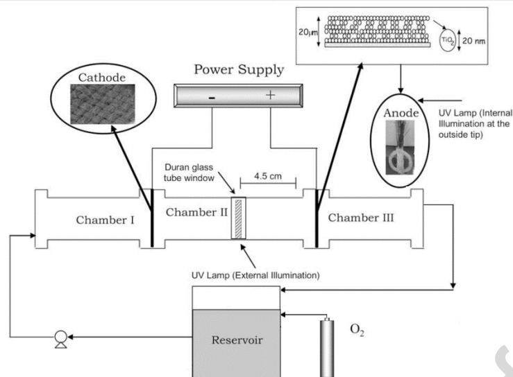
Figure 36. Schematic representation of a cylindrical continuous-flow PECR (0.64 L), constituted by three successively supplied compartments, and operating with a recycling loop. Adapted from [234]; Copyright (2009), with permission of Elsevier.
