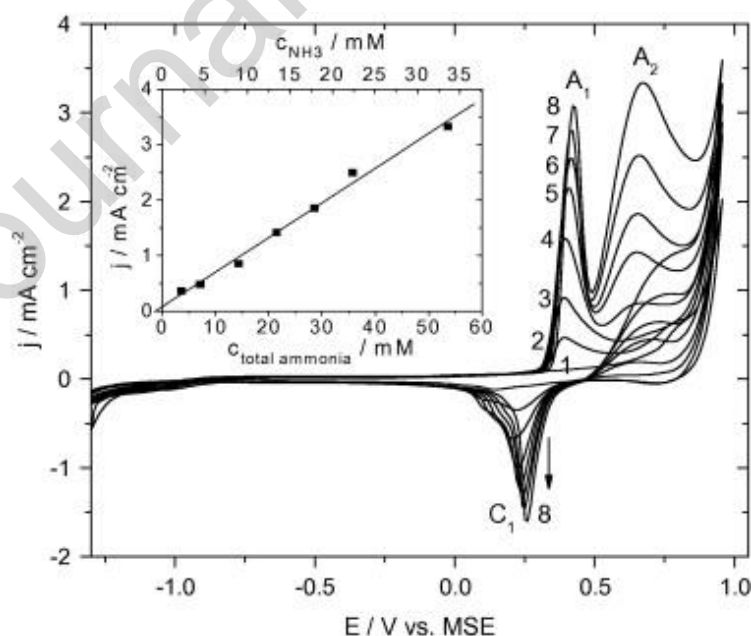
Figure 17. Cyclic voltammograms of (1) 0 mM, (2) 10 mM, (3) 20 mM, (4) 40 mM, (5) 60 mM, (6) 80 mM, (7) 100 mM, (8) 150 mM NH_4ClO_4 in 1 M NaClO_4 + NaOH at pH 9 and 25 °C, recorded on Ni electrode at 50 mV s^{-1} . Reprinted from [72], Copyright (2010), with permission of Elsevier. E (V/SHE) = E (V/Hg/Hg _2 SO _4 /sat K _2 SO _4 ) + 0.65 V.
