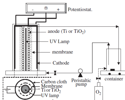
Figure 34. Schematic representation of a stirred PECR operating with a recycling loop for the analyte coupled to an O_2 absorber and used for the photo-electrochemical oxidation of the Direct Yellow-52 dye. Adapted from [232], Copyright (2006), with permission of Elsevier.
