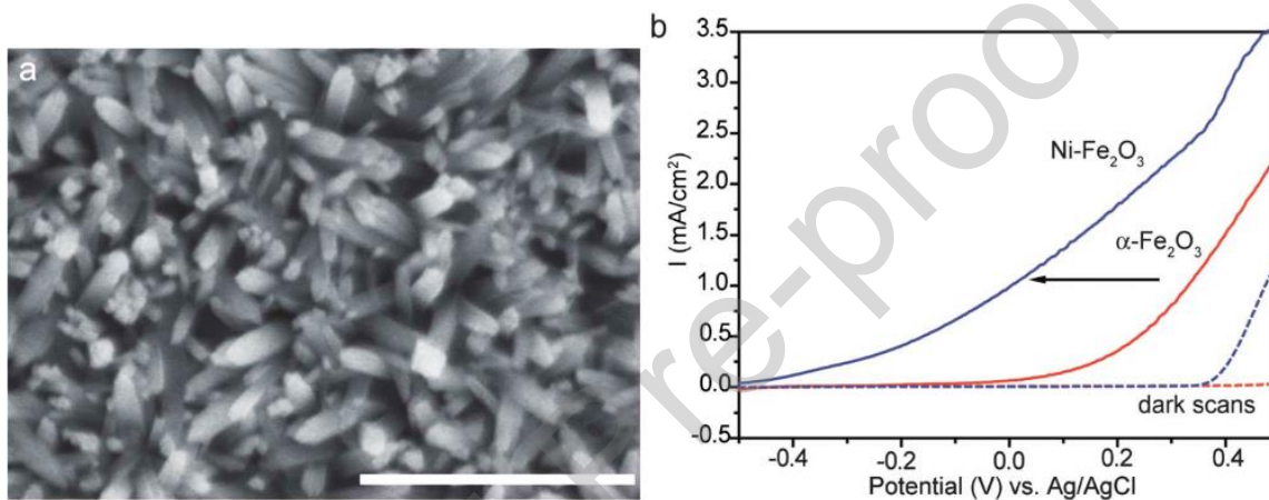
Figure 23. (a) SEM image of an array of \alpha\text{-Fe}_2\text{O}_3 nanowires on FTO; scale bar: 2 \mu\text{m} . (b) Linear scanning voltammograms (LSV) of \text{Ni-Fe}_2\text{O}_3 and \alpha\text{-Fe}_2\text{O}_3 in urea solution recorded in the dark (dotted lines) and under AM1.5G illumination. Used with permission of Royal Society of Chemistry, from [177]; permission conveyed through Copyright Clearance Center, Inc. E (V/SHE) = E (V/Ag/AgCl/sat KCl) + 0.197 \text{ V} and E (V/RHE) = E (V/Ag/AgCl/sat KCl) + 0.197 + 0.059 \cdot \text{pH} .
