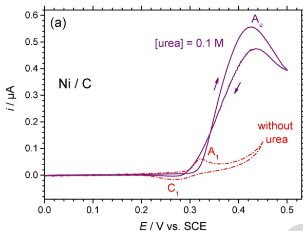
Figure 11. Voltammograms recorded for Ni/C electrode in 1 M KOH and 0.1 M urea solution, at 10 \text{ mV s}^{-1} . Reprinted from [101], Copyright (2019), with permission from Elsevier. E \text{ (V/SHE)} = E \text{ (V/SCE } 3 \text{ M KCl)} + 0.24 .
