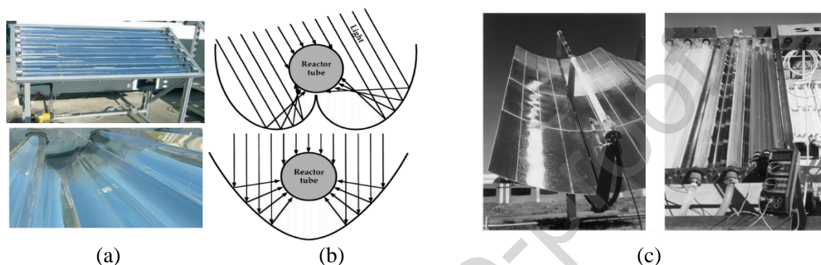
Figure 37. Pictures of typical solar photochemical reactors for water disinfection: (a) and (b) are adapted from [236]; Copyright (2011) with permission of Royal Society of Chemistry and (c) is adapted from [237]; Copyright (1999), with permission of Elsevier). (a): the reactor was made of several glass tubes (borosilicate having 90 % transmission at UV) and of polyethylene pipes and valves. The parabolic collector of the light (anodized aluminum with a high (~90 %) reflectivity in the UV range) was located around the tube. (b): Schematic solar light pathways involving direct and diffuse radiations for two different incident radiations. (c) The solar photochemical reactor for water disinfection was initially designed by Fernandez-Ibañez et al. (1999) [237].
