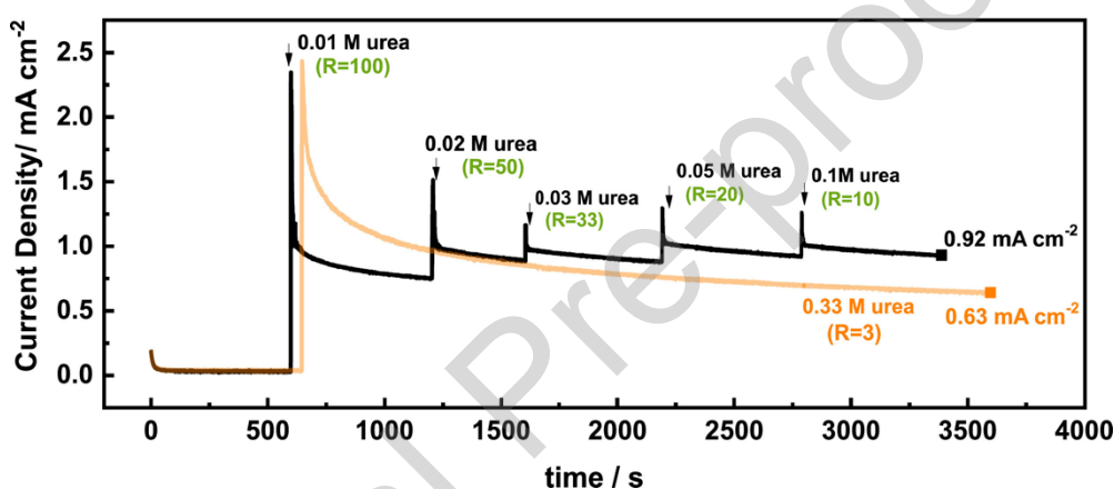
Figure 13. Chronoamperometry curves during UOR at 0.45 V vs. \text{Hg}/\text{HgO}/\text{OH}^- on NiO/NiOOH nanoparticles deposited on a rotating disk glassy carbon electrode in 1 M NaOH solution with different ratios [\text{NaOH}]/[\text{CO}(\text{NH}_2)_2] and at a rotation rate of 800 rpm. Each vertical arrow in the black plot indicates the addition of urea in the solution. Reprinted from [94], Copyright (2023), with permission from Elsevier. E (\text{V}/\text{SHE}) = E (\text{V}/\text{Hg}/\text{HgO}/1 \text{ M KOH}) + 0.14 \text{ V} .
