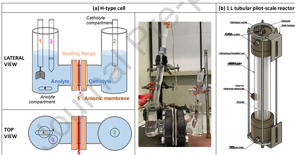
Figure 32. Scheme and pictures of the experimental reactors used for electrolysis of urea in alkaline solution. a) divided compartment cell. Working electrode (WE) and counter electrode (CE) were identified as 1 and 2. Reference electrode was labelled 3. A magnetically stirring bar (4) was used to mix the electrolyte solution. The membrane separator (5) was held in place by flanges that maintained the seal. Adapted from [136]; Copyright (2023), with permission of Elsevier. (b) Pilot scale reactor. Adapted from [86] (CC-BY 4.0 Elsevier).
