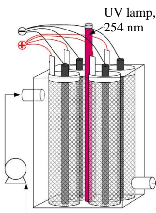
Figure 35. Schematic representation of a continuous recycling electrolyte PECR made of four undivided annular elementary cells, illuminated by an UV-C lamp located in the middle of the parallelepiped tank. The four cathodes (internal cylinders) and the four anodes (external cylindrical grids) are made of the same material (Ti – \text{IrO}_2/\text{RuO}_2 ). Adapted from [233]; Copyright (2014), with permission of Elsevier.
