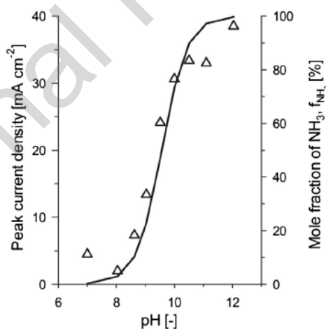
Figure 4. Correlation between peak current density associated with AOR from cyclic voltammetry on graphite electrode (triangles) and the mole fraction of ammonia (solid line) as a function of bulk pH in supporting electrolyte ( \text{NaClO}_4 1 M). Scan rate: 200 \text{ mV s}^{-1} ; T = 25 \text{ }^\circ\text{C} . Reprinted from [57], Copyright (2015), with permission from Elsevier.
