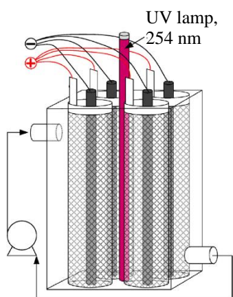
Figure 35. Schematic representation of a continuous recycling electrolyte PECR made of four undivided annular elementary cells, illuminated by an UV-C lamp located in the middle of the parallelepiped tank. The four cathodes (internal cylinders) and the four anodes (external cylindrical grids) are made of the same material (Ti – \text{IrO}_2/\text{RuO}_2 ). Adapted from [233]; Copyright (2014), with permission of Elsevier.
