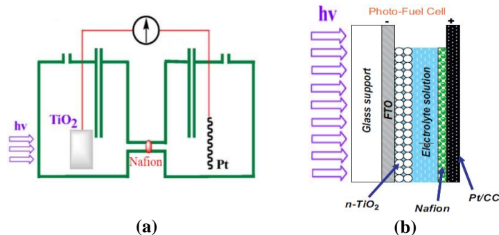
Figure 31. Schematic representation of two types of lab-scale PECR, built with the same anode (nanocrystalline titanium ( n\text{-TiO}_2 ) deposited on a FTO) and devoted to organics oxidation via the generated photocurrent. In Figure (a) (Adapted from [197]; Copyright (2009), with permission of Elsevier), the cathode was introduced into a separated compartment, while in Figure (b) (Adapted from [224]; Copyright (2010), with permission of Elsevier), the composite type cathode (Nafion graphite porous media) was located into the single compartment of the cell.
