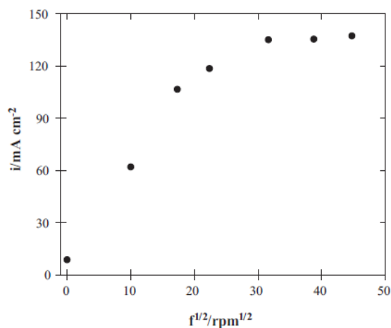
Figure 15. Levich plot on Ni electrode in 0.33 M urea and 5 M KOH solution using a RDE at various rotation speeds: 100, 300, 500, 1000, and 1500 rpm. Reprinted from [124], Copyright (2012), with permission from Elsevier.
