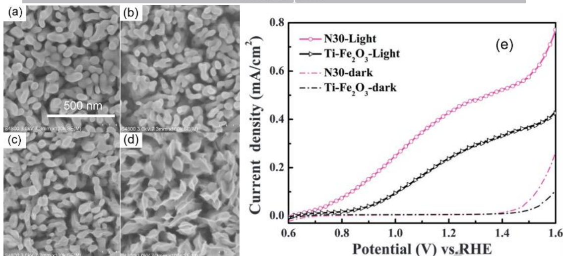
Figure 24. Plan view SEM images of (a) Ti-Fe 2 O 3 , plus Ni(OH) 2 electrodeposited for a time of (b) 120, (c) 300 and (d) 600 s. (e) Line scan voltammograms for Ti-Fe 2 O 3 and Ti-Fe 2 O 3 /Ni(OH) 2 (30 s deposition) in the dark (dashed lines) and under illumination (line + symbol). NaOH 1 M with 0.1 M urea. Scan rate: 10 mV s -1 . Illumination: 100 mW cm -2 . Reprinted from [179]; Copyright (2015), with permission from Elsevier.
