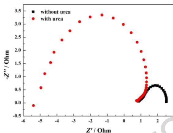
Figure 9. Nyquist plots of nickel nanowire array electrode at 0.47 V vs. Ag/AgCl/Cl - in 5 M KOH solution in the presence and the absence of 0.33 M urea. Reprinted from [96], Copyright (2016), with permission from Elsevier. E (V/SHE) = E (V/Ag/AgCl/3 M KCl) + 0.197 V.
