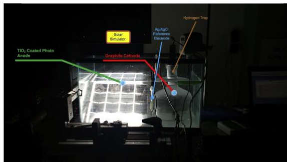
Figure 33. Experimental setup of the PECR with \text{TiO}_2 photoanode used by Chehade et al. (2018) for \text{H}_2 production. Reprinted from [228]; Copyright (2018), with permission of Elsevier.
