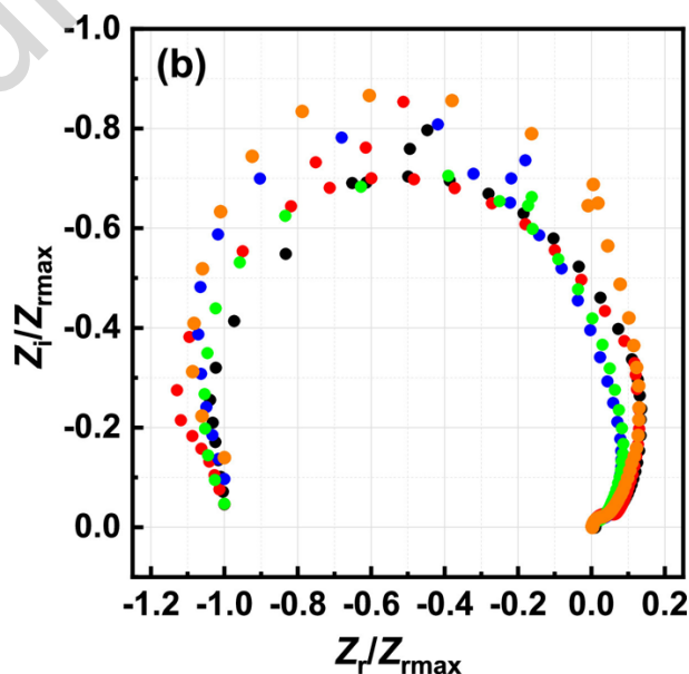
Figure 10. Nyquist plots corresponding to EIS spectra obtained on NiO/NiOOH NPs at 800 rpm and 0.53 V vs. Hg/HgO/OH - . Solution composition: 5 M NaOH and 0.01 M urea (black plot) and in the presence of 0.01 M CO 3 2- (red plot), 0.01 M NO 2 - (blue plot), 0.01 M ·OCN (green plot), or 0.01 M NH 3 (orange plot) in solution.
