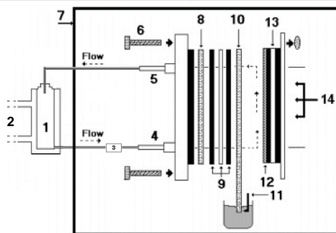
Figure 38. Schematic representation of an undivided filter press PECR: (1) continuously recycled electrolyte's tank; (2) thermoregulated fluid; (3) pump; (4)/(5) electrolyte inlet and outlet; (6) screw; (8) photoanode ( \text{Ti/Ru}_{0.3}\text{Ti}_{0.7}\text{O}_2 ); (9) Teflon gaskets for studying the effect of the thickness of the electrolytic compartments; (10) IONAC® membrane acting as ionic conductor for the reference electrode (11); (12) cathode: Ti-mesh; (13) quartz glass; (14) Incident UV light produced by a mercury lamp ( 4.2 \text{ kW m}^{-2} emitted at 254 nm). Adapted with permission from [238]; Copyright (2007), American Chemical Society.
