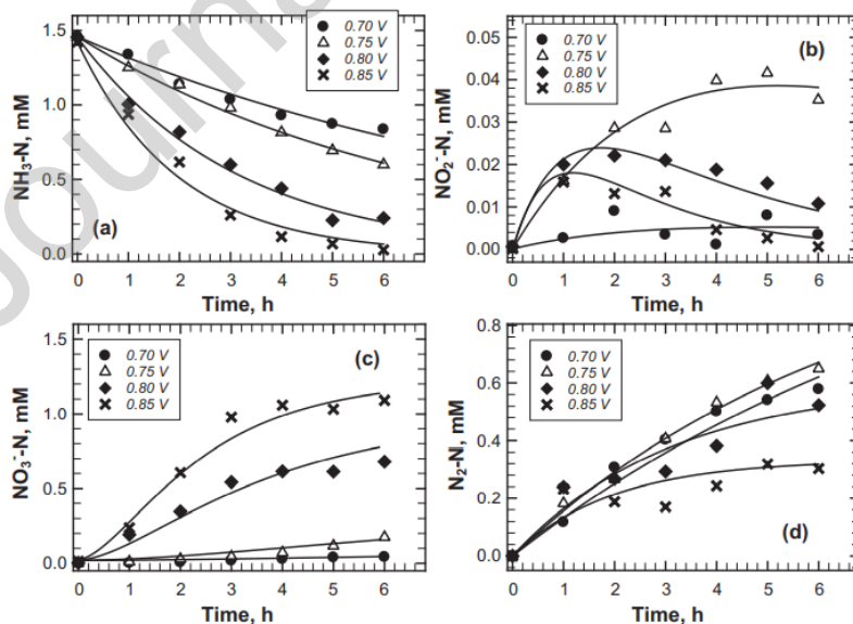
Figure 5. Concentration changes of nitrogen species (a) NH_3-N , (b) NO_2^-N , (c) NO_3^-N , (d) N_2-N during batch electrolysis at constant potentials of 0.7-0.85 V vs. Hg/HgO/OH - on nickel foam electrode as a function of reaction time. Initial [NH_3-N] = 20 ppm, pH = 11, 0.1 M Na_2SO_4 . Reprinted from [73], Copyright (2018), with permission of Elsevier. E (V/SHE) = E (V/Hg/HgO/1 M KOH) + 0.14 V.
