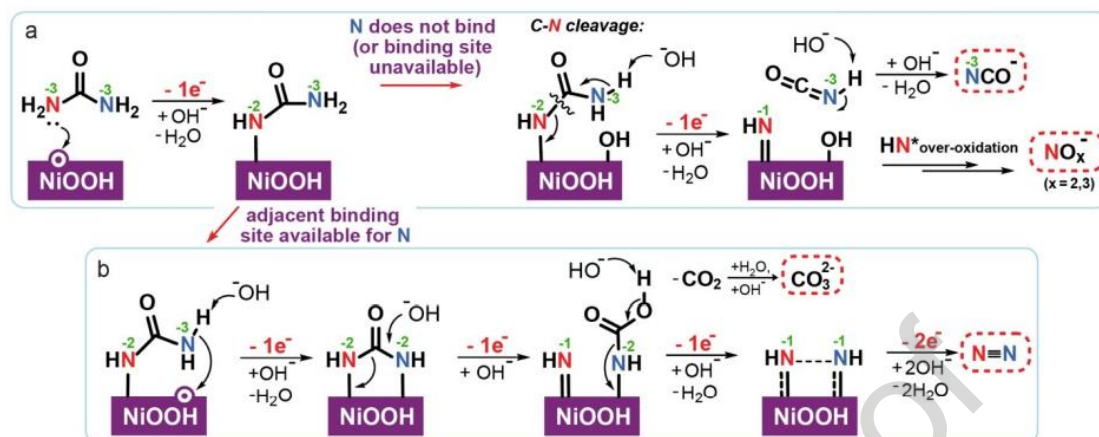
Figure 21. Proposed reaction pathways for UOR from Tatarchuk et al. Reprinted from [76], Copyright (2022), with permission from John Wiley and Sons.
