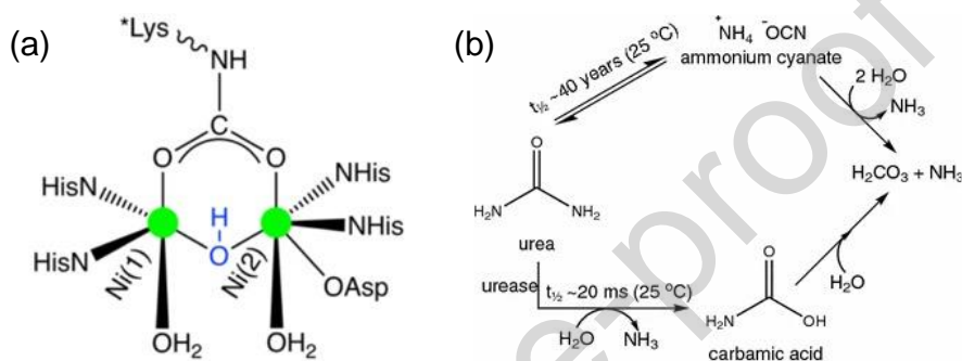
Figure 2. (a) Urease enzyme representation. Adapted from [18], with permission from John Wiley and Sons. (b) Urea chemical and enzymatic decomposition pathways. Reprinted from [16], with permission from Springer Nature BV.
