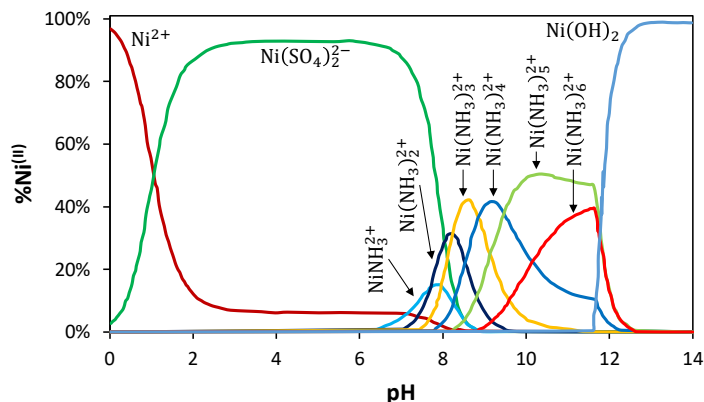
Figure 20. Predominance distribution–pH diagram for 0.01 M \text{Ni}^{2+} and 1.0 M (\text{NH}_4)_2\text{SO}_4 in solution. Adapted from [147] Copyright (2006), with permission from Elsevier.
