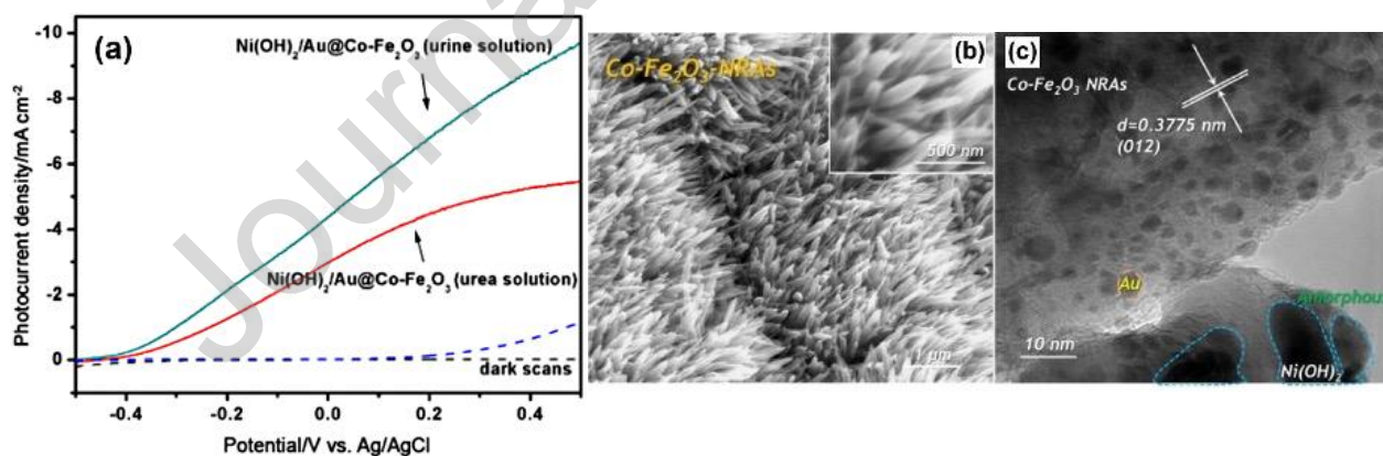
Figure 25. (a) Line-scan voltammograms of a Ni(OH) 2 /Au@Co-Fe 2 O 3 photoanode in urea solution and human urine solution in the dark (dashed lines) and under AM1.5G illumination (100 mW cm -2 ) (solid lines). (b) SEM and (c) TEM images of a Ni(OH) 2 /Au@Co-Fe 2 O 3 photoanode. Reprinted from [180]; Copyright (2019), with permission from Springer Nature. E (V/SHE) = E (V/Ag/AgCl/sat KCl) + 0.197 V.
