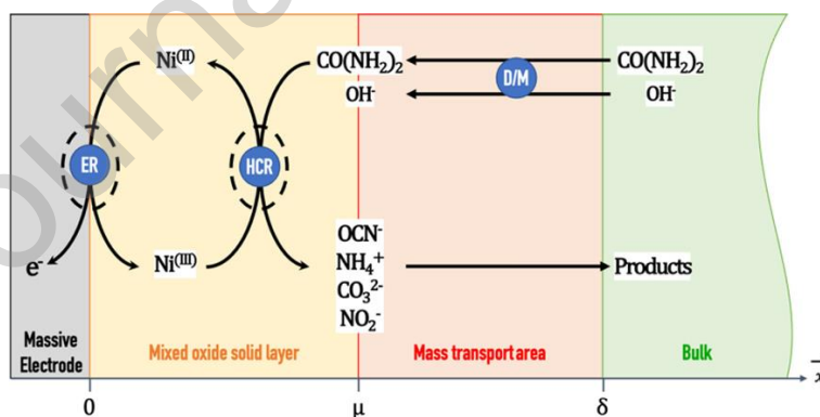
Figure 12. Schematic representation of the indirect oxidation of urea on NiOOH/Ni(OH) 2 operating on the surface of a massive nickel anode in alkaline medium. ER, HCR, and D/M respectively refer to the NiOOH Electrogeneration Reaction, to the Heterogeneous Catalytic Reaction and to the mass transport by Diffusion and Migration. Reprinted from [136], Copyright (2023), with permission from Elsevier.
