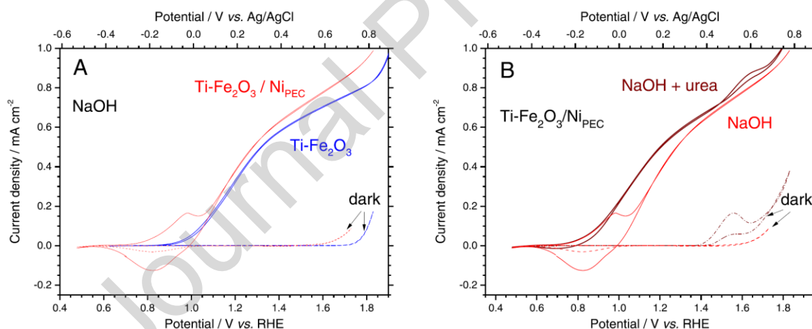
Figure 27. Voltammetry in the dark and under illumination of (A) FTO/Ti-Fe 2 O 3 in NaOH, before and after PEC deposition of NiOOH (8.75 mC cm -2 ); (B) Ti-Fe 2 O 3 /NiPEC in NaOH, with or without urea. [NaOH] = 1 M; [urea] = 0.33 M. Scan rate: 10 mV s -1 . Illumination: AM1.5G, 1000 W m -2 . Reprinted from [37]; Copyright (2023), with permission of Elsevier.
