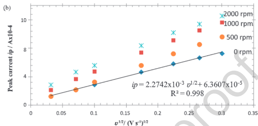
Figure 18. i_p (peak current) for the AOR vs. v^{1/2} (potential scan rate) at different angular velocities (0, 500, 1000 and 2000 rpm) in a 0.1 M KOH and 0.01 M \text{NH}_4\text{Cl} solution. Reprinted from [71], Copyright (2013), with permission from Elsevier. E (V/SHE) = E (V/Hg/HgO/1 M KOH) + 0.14 V.
