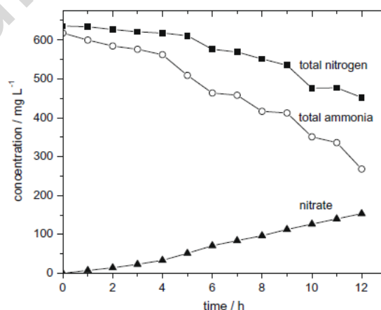
Figure 19. Reactant and product concentration temporal evolution during the ammonia electrolysis on NiOOH at 20 \text{mA cm}^{-2} . Solution composition: 50 mM \text{NH}_4\text{ClO}_4 + 1 M \text{NaClO}_4 + NaOH at pH 11. Reprinted from [72], Copyright (2010), with permission of Elsevier. E (V/SHE) = E (V/Hg/Hg 2 SO 4 /sat K 2 SO 4 ) + 0.65 V.
