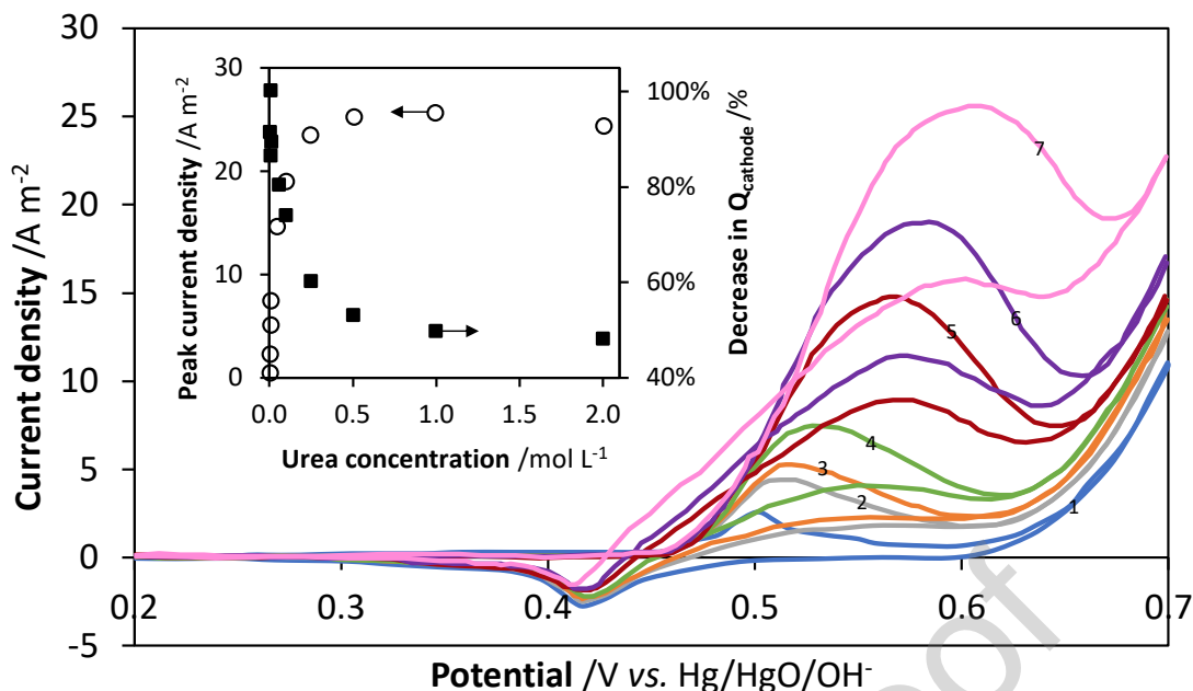
Figure 14. Cyclic voltammetry on Ni electrode at a scan rate of 10 \text{ mV s}^{-1} in 1 M KOH solution with variable urea concentration: (1) 0 M, (2) 0.05 M, (3) 0.1 M, (4) 0.2 M, (5) 0.3 M, (6) 0.4 M, and (7) 0.5 M. Insets: Changes in anodic peak current density and the decrease in cathodic charge at various urea concentrations. Adapted from [124], Copyright (2012), with permission from Elsevier. E \text{ (V/SHE)} = E \text{ (V/Hg/HgO/1 M KOH)} + 0.14 \text{ V} .
