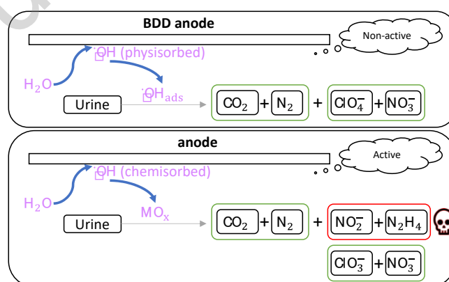
Figure 3. Schematic representation of UOR in artificial human urine at neutral pH on either BDD or \text{IrO}_2 anodes. Adapted from [54], Copyright (2015), with permission from Elsevier.
