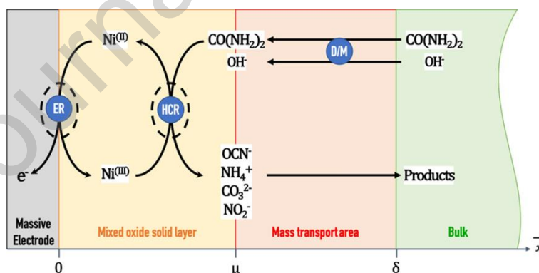
Figure 12. Schematic representation of the indirect oxidation of urea on NiOOH/Ni(OH) 2 operating on the surface of a massive nickel anode in alkaline medium. ER, HCR, and D/M respectively refer to the NiOOH Electrogeneration Reaction, to the Heterogeneous Catalytic Reaction and to the mass transport by Diffusion and Migration. Reprinted from [136], Copyright (2023), with permission from Elsevier.
