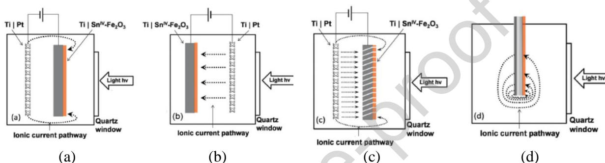
Figure 41. Schematic representation of the current pathways as function of the geometry of the PECR, and in particular of the relative position of the electrodes with respect to the light source (Reprinted from [204]; Copyright (2016), with permission of Royal Society of Chemistry).
