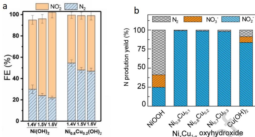
Figure 6. (a) Faradaic efficiencies (FEs) of the major products of potentiostatic urea electrolysis of 0.33 M urea in 1 M KOH solution on Ni(OH) 2 and Ni 0.8 Cu 0.2 (OH) 2 electrodes at different applied potential vs. RHE. Reprinted from [76], Copyright (2022), with permission from John Wiley and Sons. (b) Yield ratio of N products during potentiostatic ammonia electrolysis at 1.53 V vs RHE in 10 -3 M NH 3 and 0.1 M KOH solution on Ni x – Cu 1-x oxyhydroxide with different x (x=0-1). Reprinted from [59], Copyright (2020), with permission from Elsevier.
