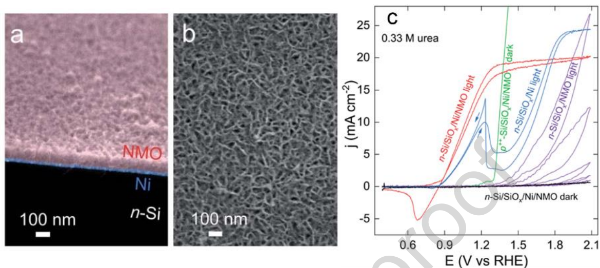
Figure 29. (a) Tilted SEM cross-section color image of an (n)c-Si/SiO x /Ni/NMO surface ; (b) Top view SEM image of an (n)c-Si/SiO x /Ni/NMO surface. (c) Voltammograms recorded in 1 M KOH + 0.33 M urea in the dark on (n)c-Si/SiO x /Ni/NMO (black curve) and (p ++ )-Si/SiO x /Ni/NMO (green curve) and under illumination on (n)c-Si/SiO x /NMO (purple curve, 5 consecutive cycles), n-Si/SiO x /Ni (blue curve), and (n)c-Si/SiO x /Ni/NMO (red curve). Scanning speed 100 mV s -1 , solar illumination (100 mW cm -2 , AM 1.5G). Reprinted from [194]; Copyright (2013), with permission of Royal Society of Chemistry.
