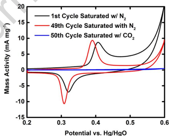
Figure 8. \text{LaNiO}_3 supported on Vulcan carbon cycled 49 times in an \text{N}_2 -saturated solution of 5 M KOH. The 50th cycle was performed in the same electrolyte saturated with \text{CO}_2 . All cycles were performed with a scan rate of 100 \text{ mV s}^{-1} . All currents were normalized by the mass of the perovskite drop-cast on the electrode (in mg) to obtain mass activities. Reprinted with permission from [88], Copyright (2016) American Chemical Society. E \text{ (V/SHE)} = E \text{ (V/Hg/HgO/1 M KOH)} + 0.14 \text{ V} .
