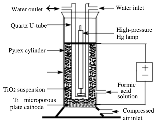
Figure 30. Schematic representation of discontinuous slurry PECR stirred by sparged air, used for formic acid photoelectrochemical degradation. The outer cylindrical Pyrex casing was 55 mm in diameter and 250 mm in height. The thickness of the annulus containing \text{TiO}_2 particle suspension was 5 mm. Adapted from [201]; Copyright (2002), with permission of Elsevier.
